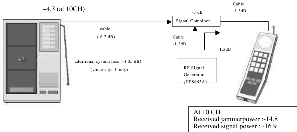
Figure 1: Test Setup
