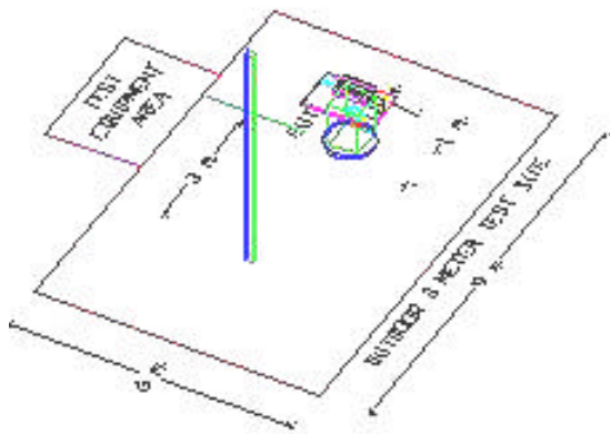
Figure 2. Diagram of 3-meter outdoor test range
