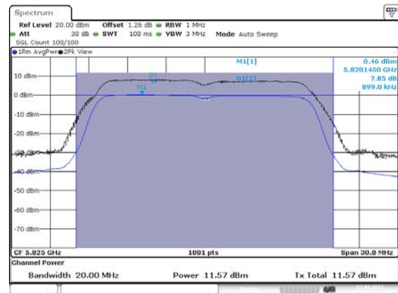
11A5.8G-20M – F3 [Port 2]
