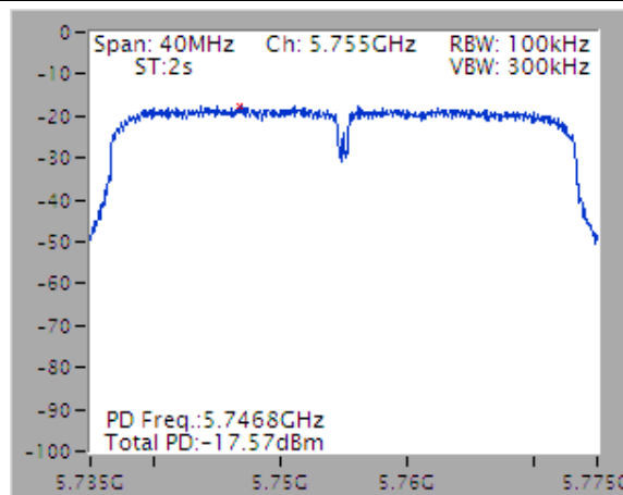
11N5.8G-40M – F4 [Sum All Chains]
