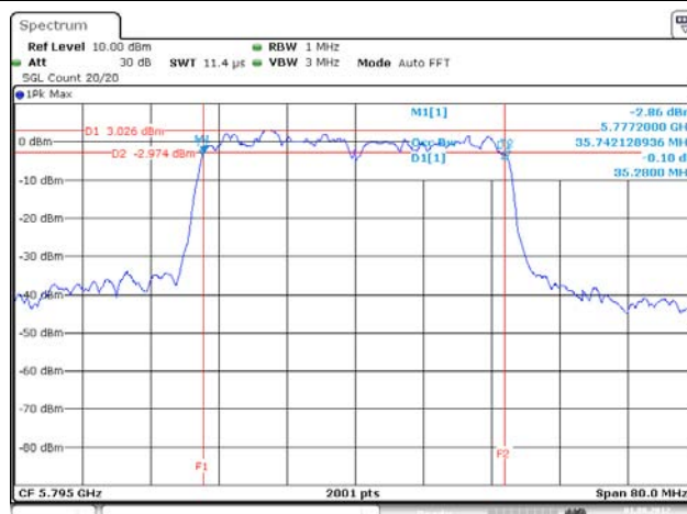
11N5.8G-40M – F5 [Port 2]
