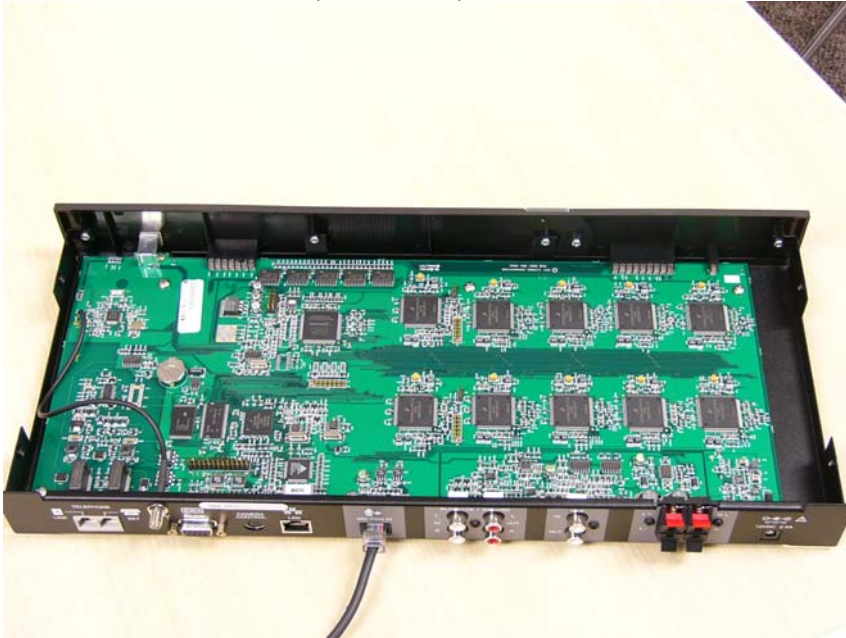
Rav 900 Internal Photo (Rear View)
