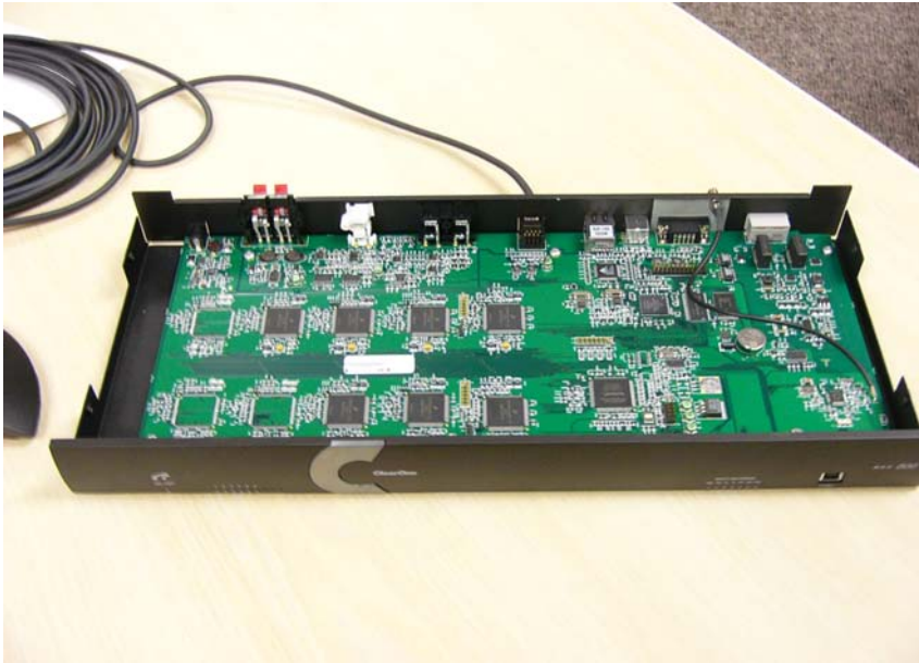
Rav 600 Internal Photo (Rear View)
