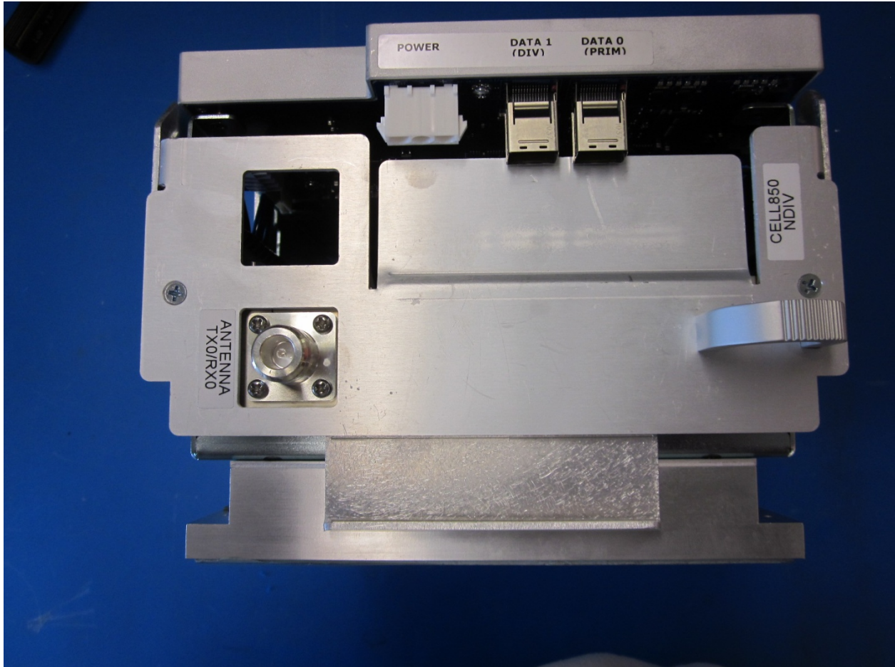
RF Module Assembly #1
