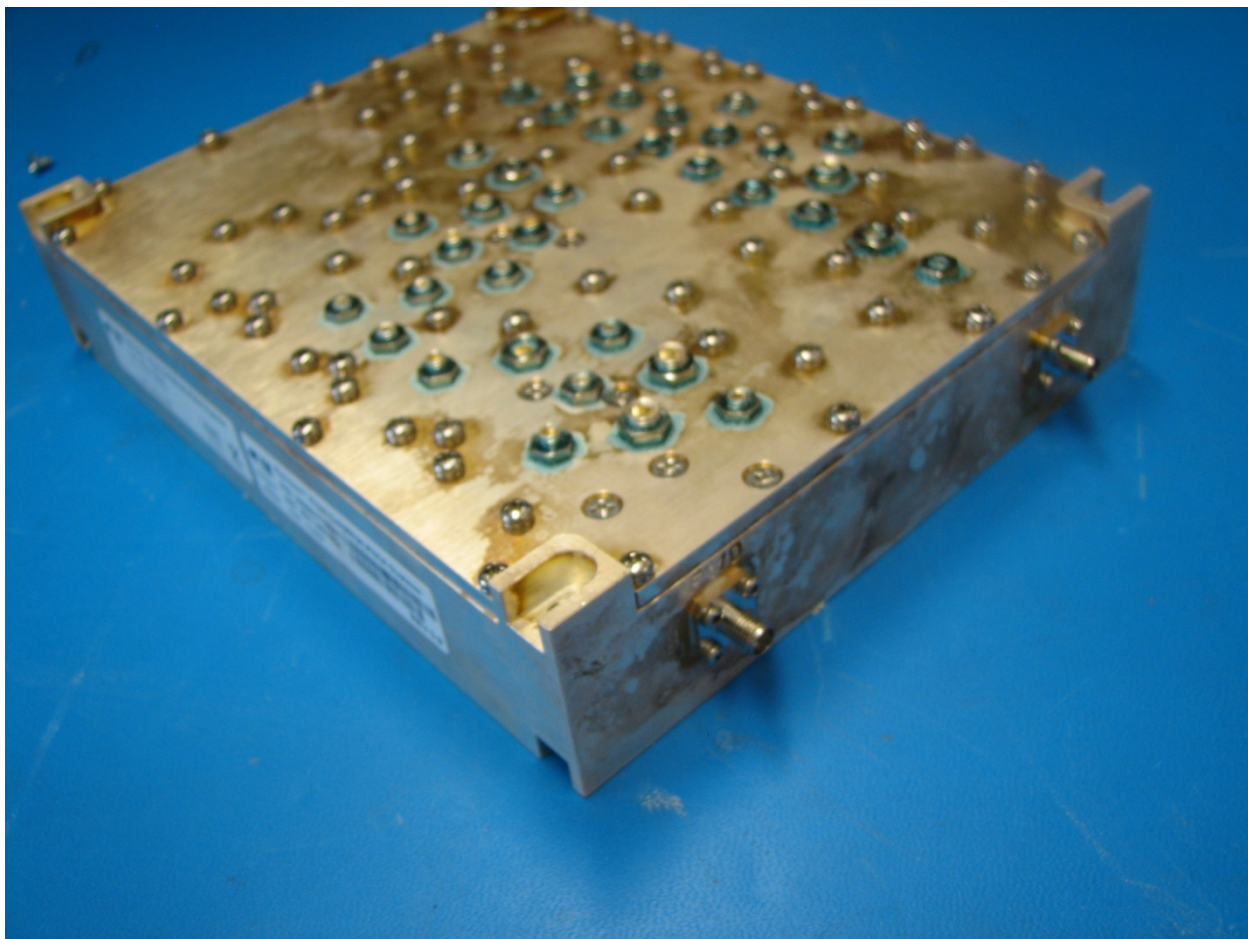
Duplexer #3
