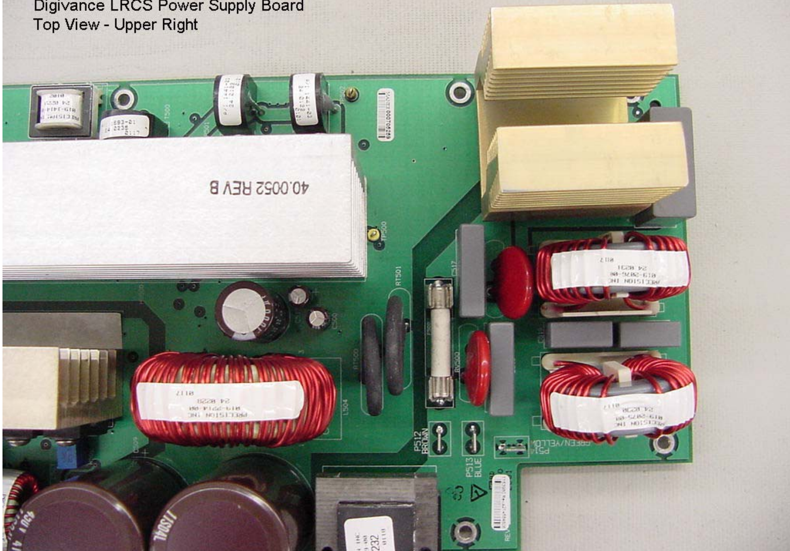
Digivance LRCS 1300-Watt Power Supply Top View 5
