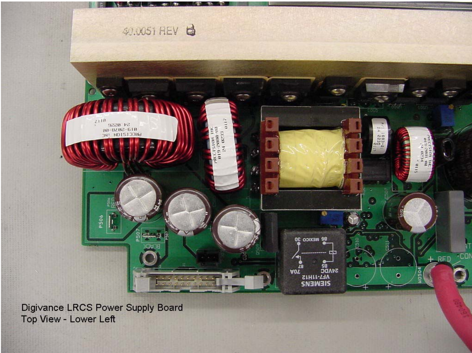
Digivance LRCS 1300-Watt Power Supply Top View 1
