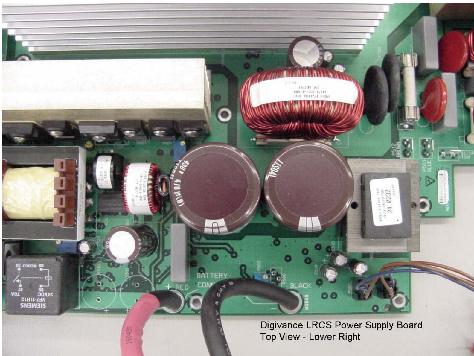
Digivance LRCS 1300-Watt Power Supply Top View 2
