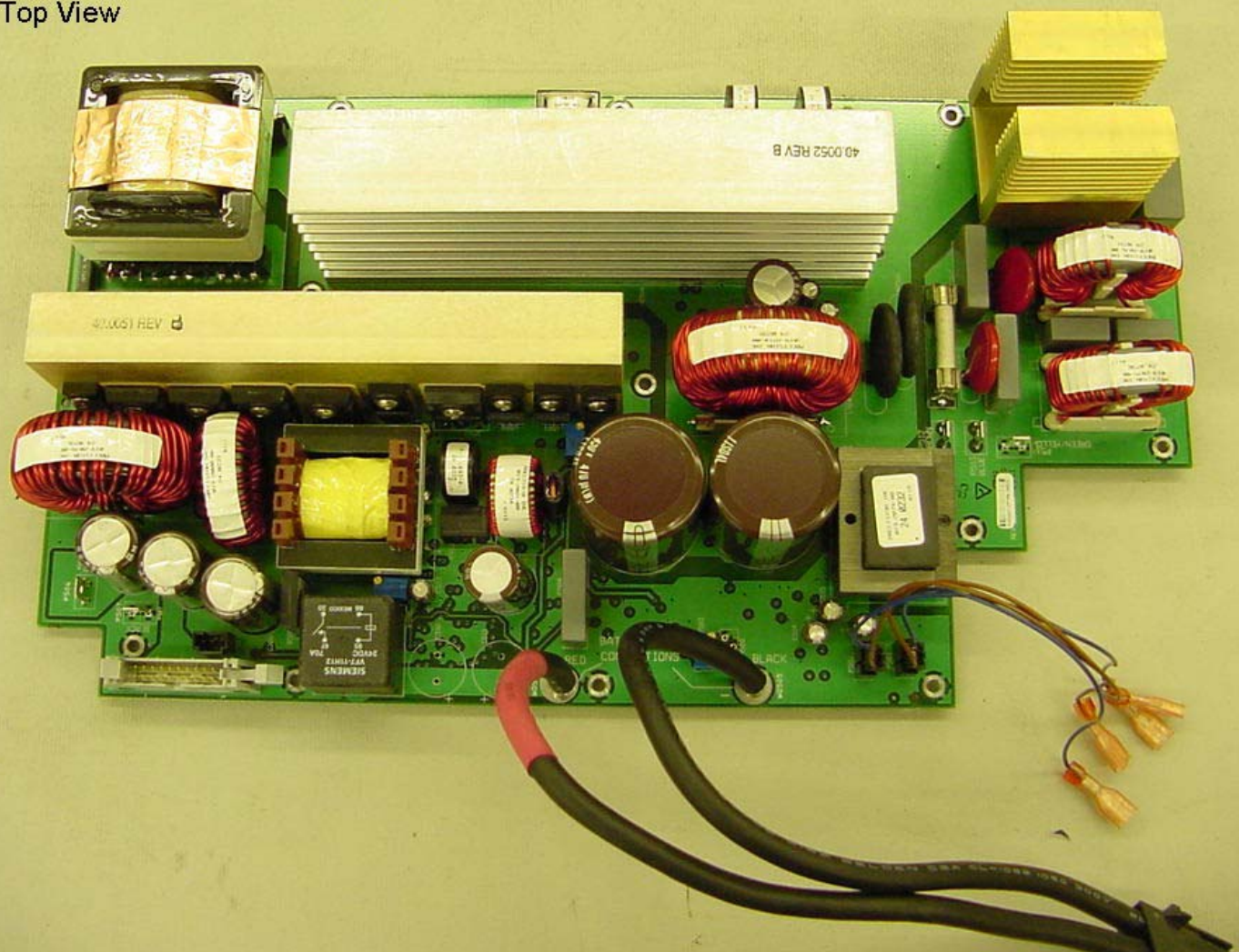
Digivance LRCS 1300-Watt Power Supply Top View
