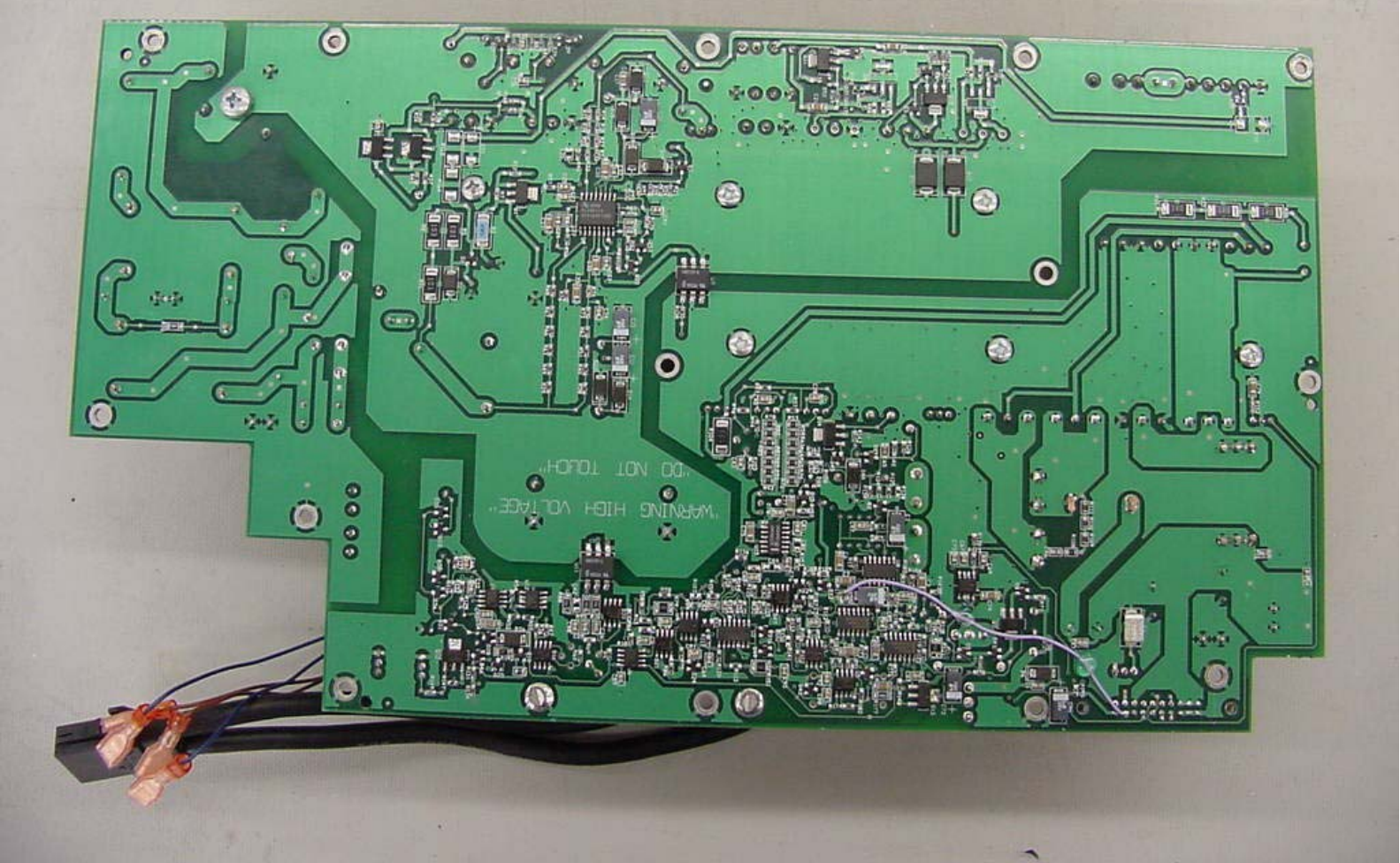
Digivance LRCS 1300-Watt Power Supply Bottom View
