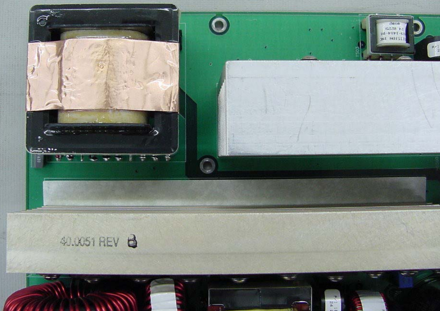
Digivance LRCS 1300-Watt Power Supply Top View 3
