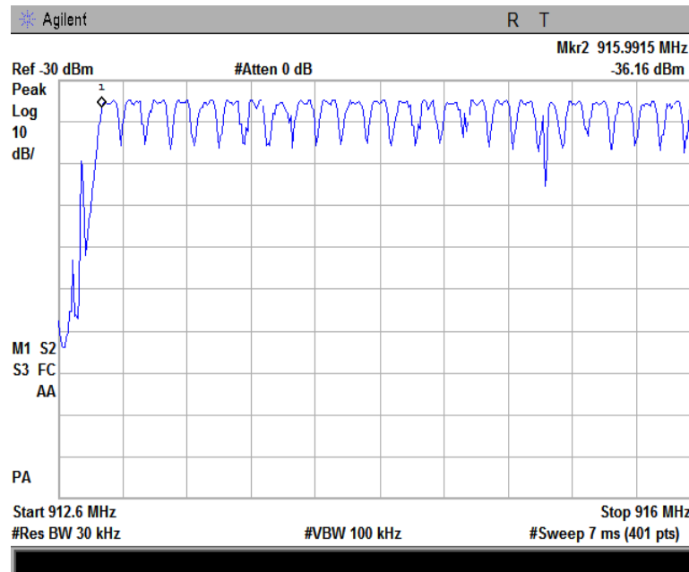
Plot 7.3.2 Number of hopping frequencies
