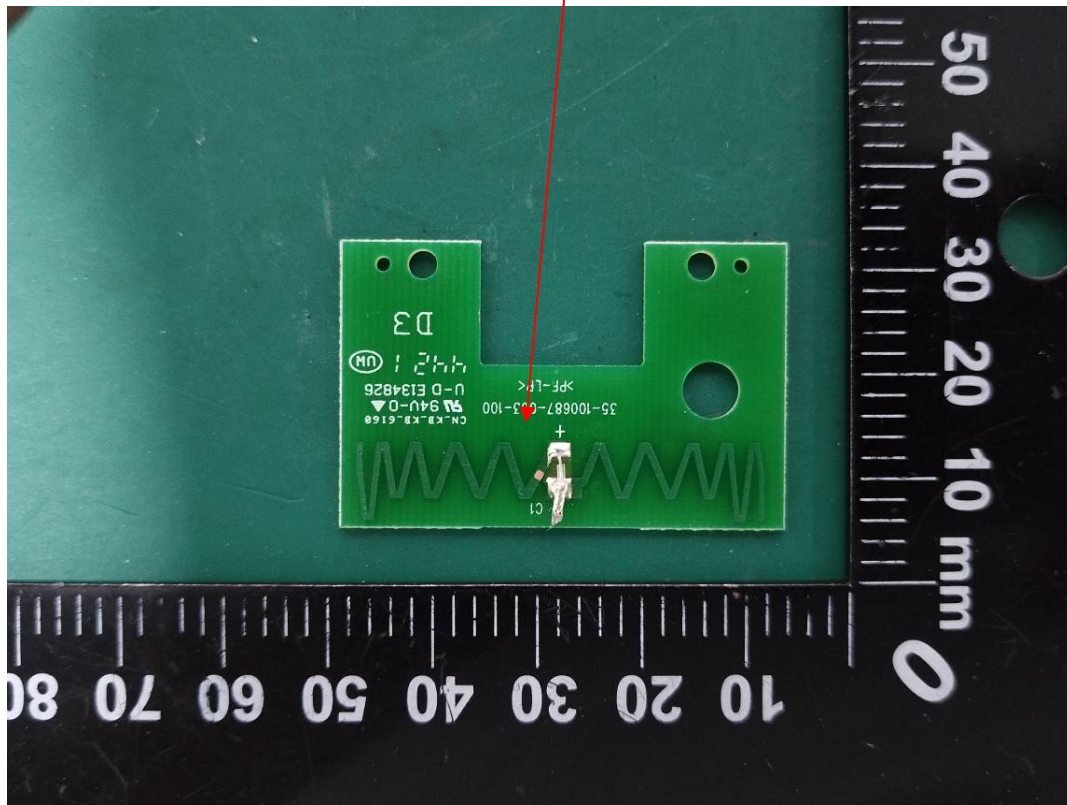
DECT ANT 0
