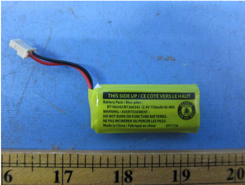
Figure 4 - 2.4V 750mAh GPI Ni-MH rechargeable battery
