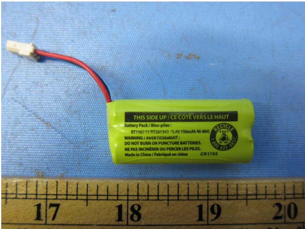
Figure 4 - 2.4V 750mAh Corun Ni-MH rechargeable battery
