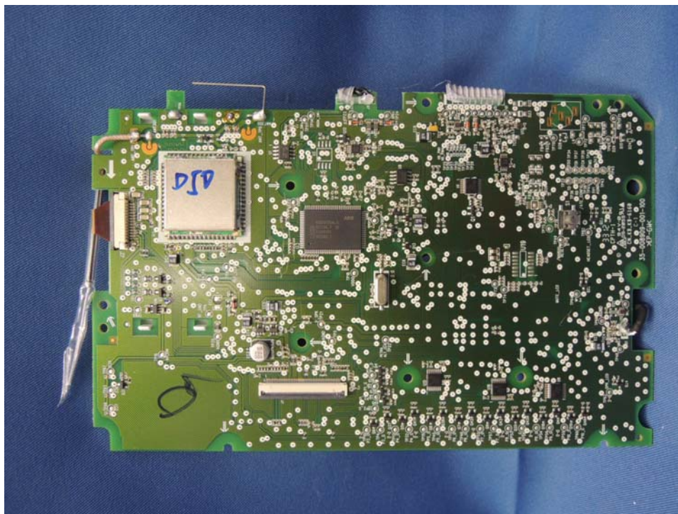
Deskset LCD Display rear side (View 1)
