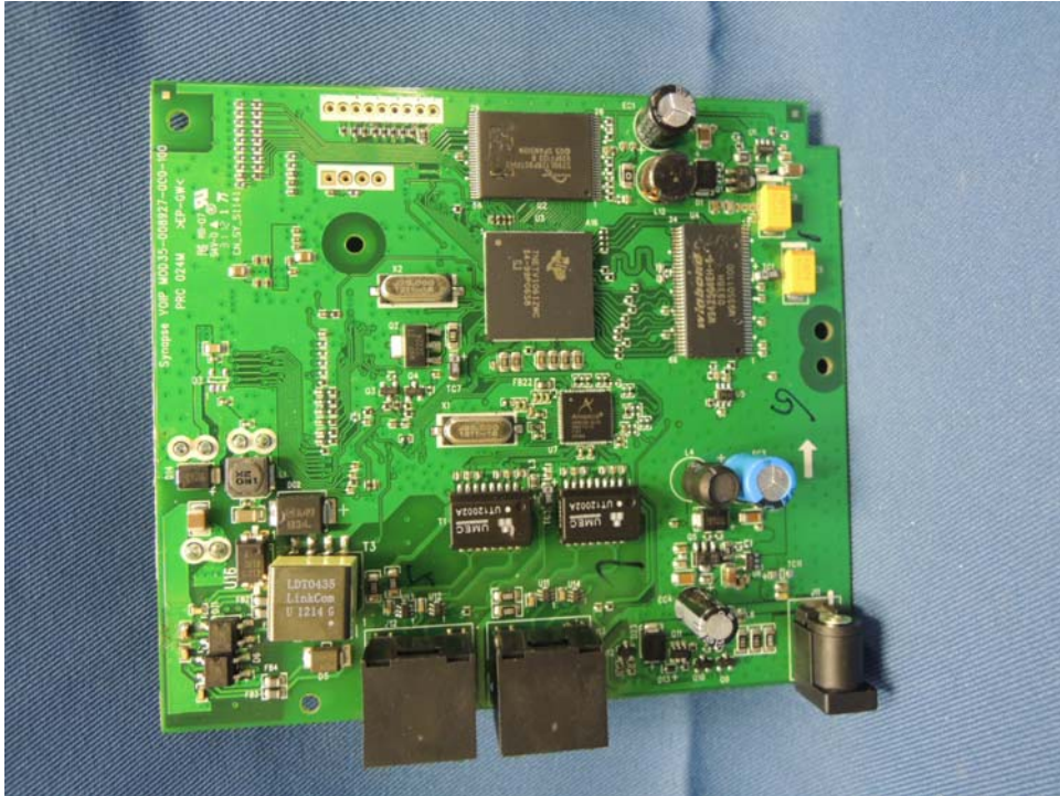
Deskset Main PCB comp side (View 2)
