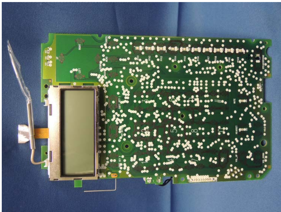
Deskset LCD Display front side (View 1)
