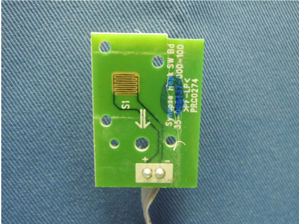
Deskset Page Key front side
