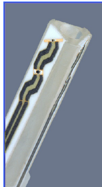
Figure 2. E-field Probe
