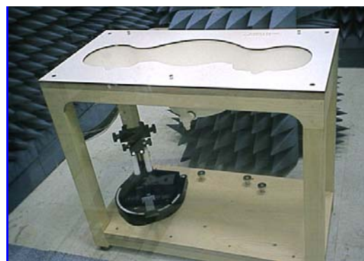
Figure 5. SAM Twin Phantom
