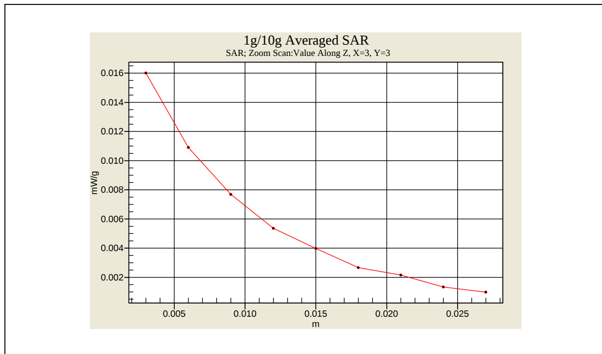
Brain SAR Measurement _ CH2
