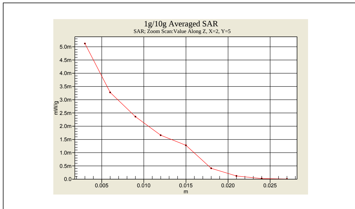
Body SAR Measurement _ CH2 _ Muscle
