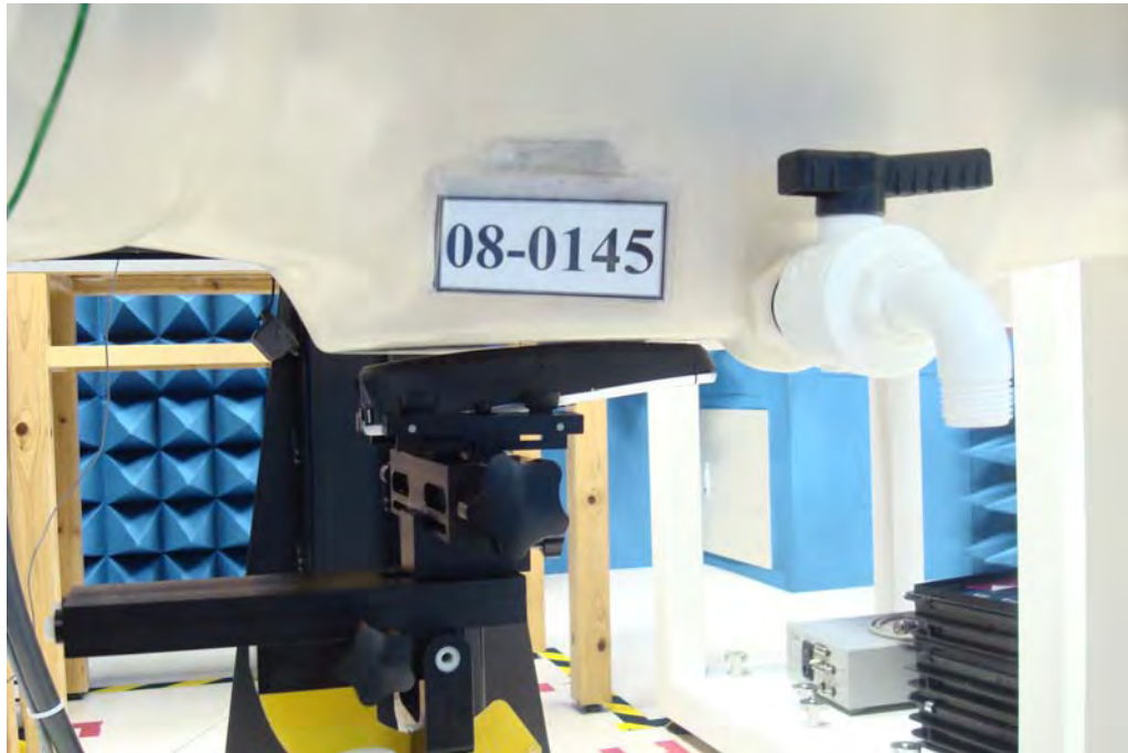
Figure 18. Body SAR Test Setup _ Back to Phantom 0mm separation
