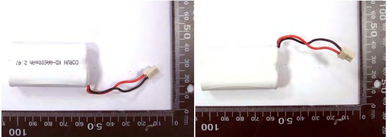
Figure 2. Battery (Ni-Cd 2.4V , 600mAh)
