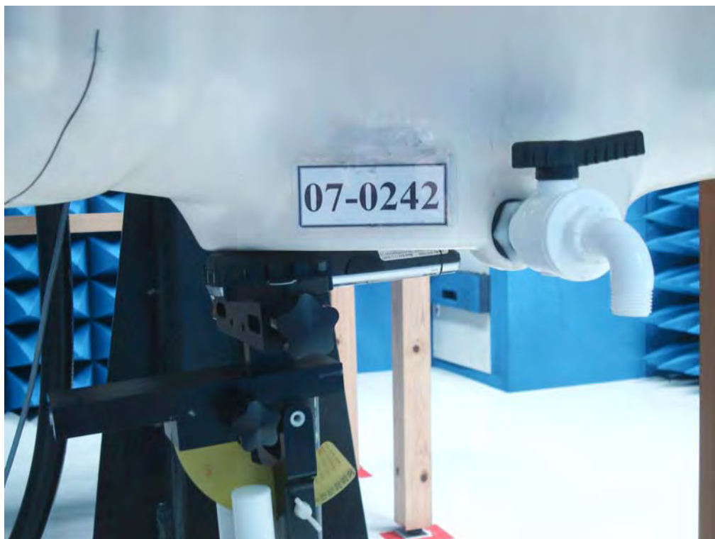
Figure 19. Body SAR Test Setup (Flat Section)
