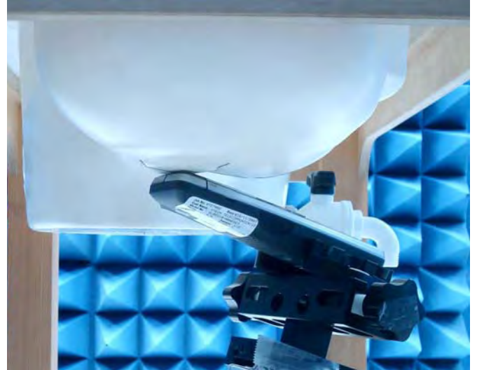
Figure 16.Right Head SAR Test Setup (Tilted)
