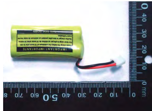
Figure 3. Battery (Ni-MH 2.4V , 600mAh)
