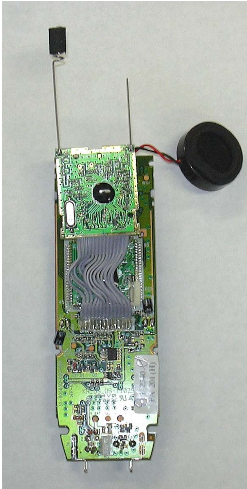
Vtech T2326/T2340 Handset PCB
