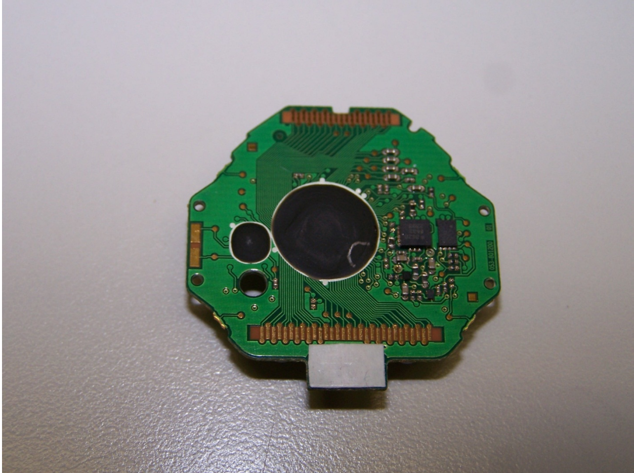
Figure 3: Front View of watch module without display.
