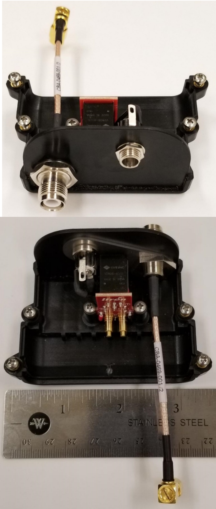
More of the base snap on feature (IMRB-EXT only)
