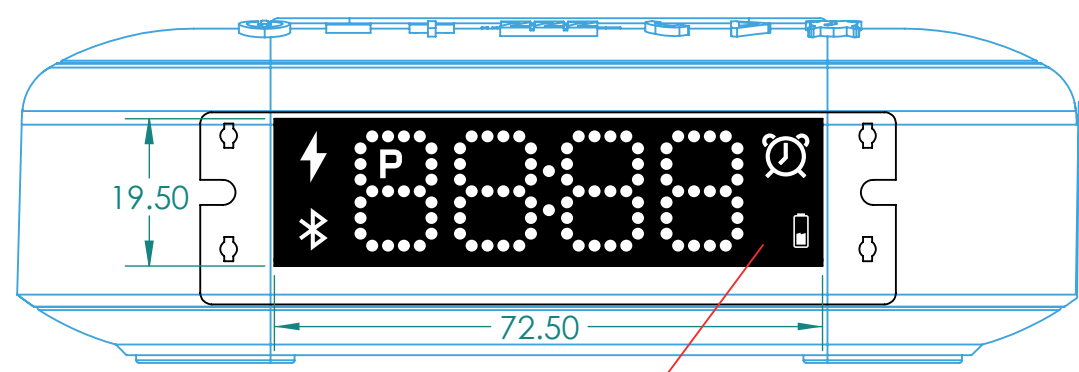
LED Display LCD Display Viewing Area - 72.5mm x 19.5mm
