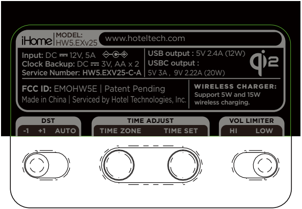
Label - same quality as current sample_ ShuoYu actual size: 72.2W x 28.8H (mm)
