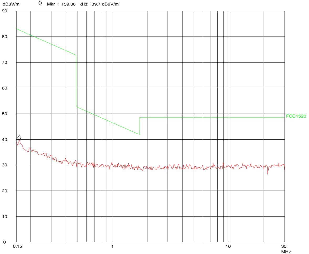
Spurious Emissions 0.15 - 30 MHz, Peak Detector
