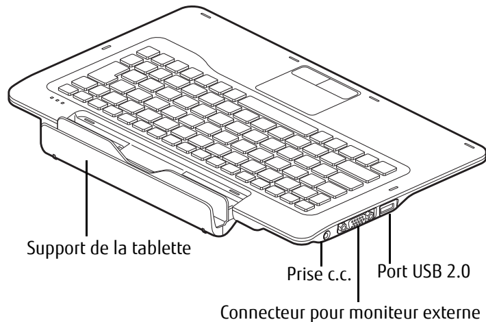
Figure 22. Station d'arrimage - arrière
