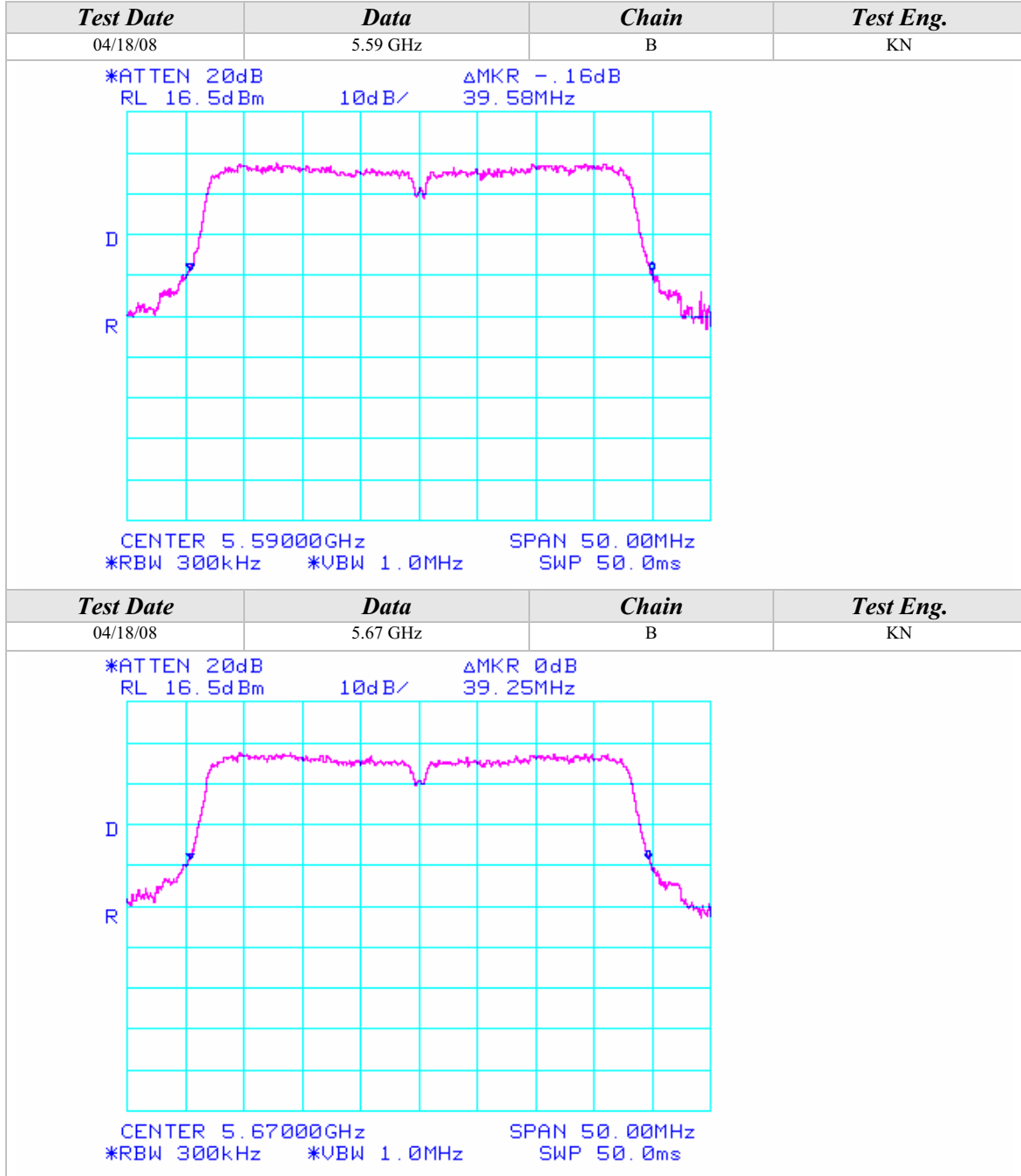
802.11n Mode, 5GHz, 40MHz Wide
