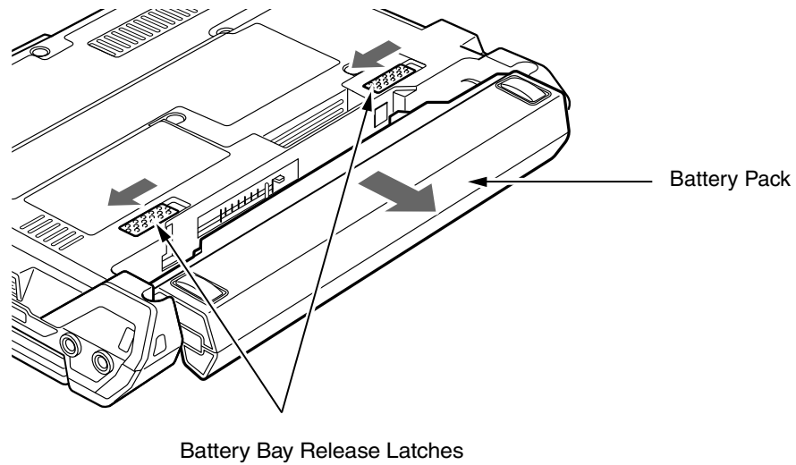
Figure 28. Removing a Battery
