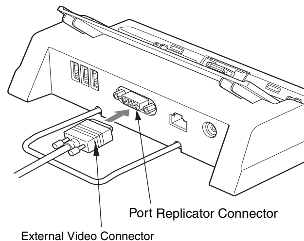
Figure 35. Connecting to Port Replicator
