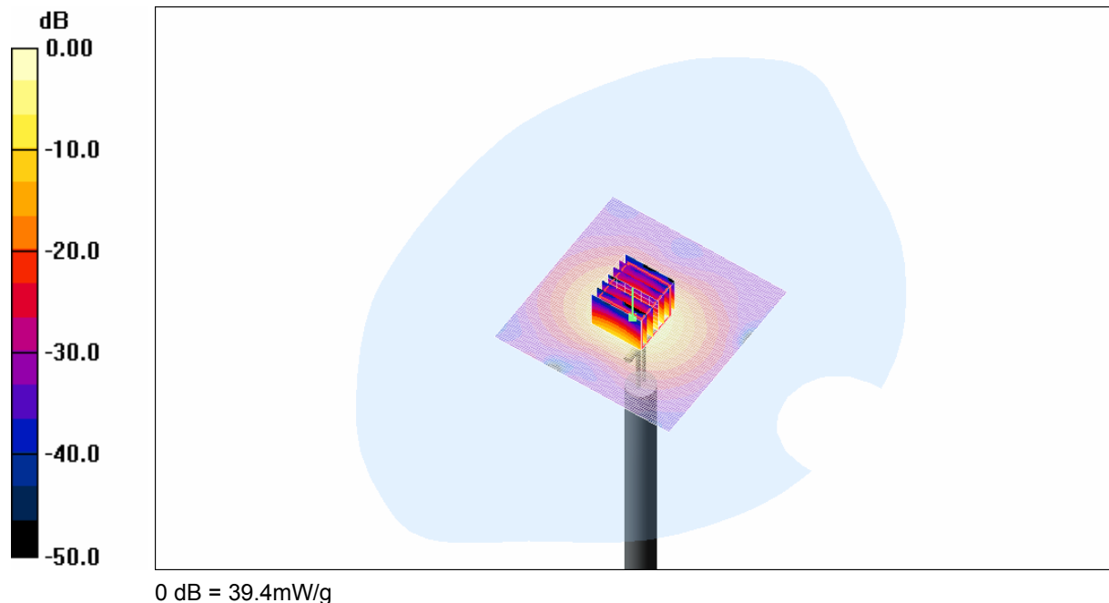
SAR MEASUREMENT PLOT 61
