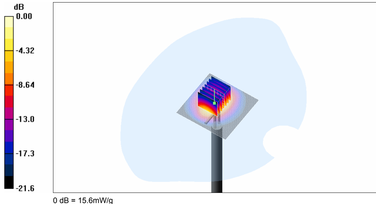
SAR MEASUREMENT PLOT 60
