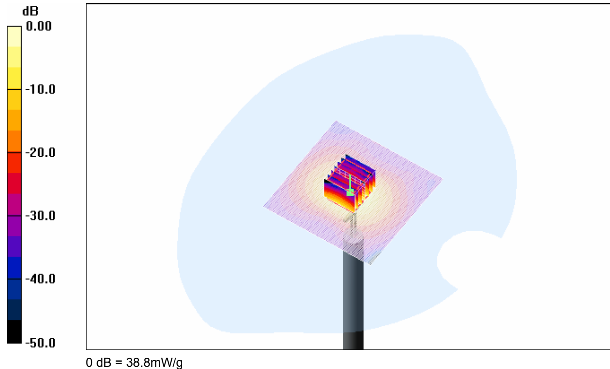
SAR MEASUREMENT PLOT 62
