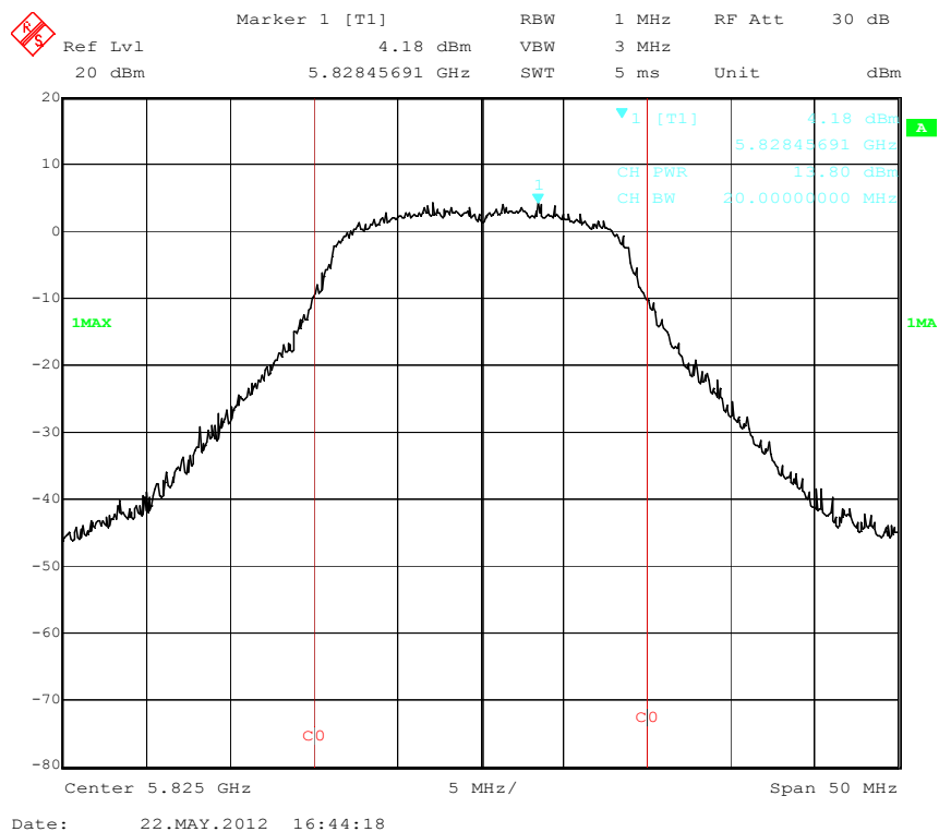
Output Power High Channel (802.11n-20MHz 5.7GHz)
