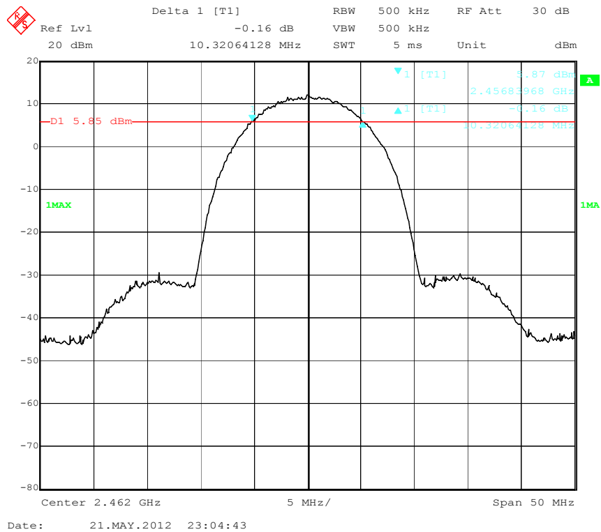
6 dB Bandwidth – 802.11b, High Channel
