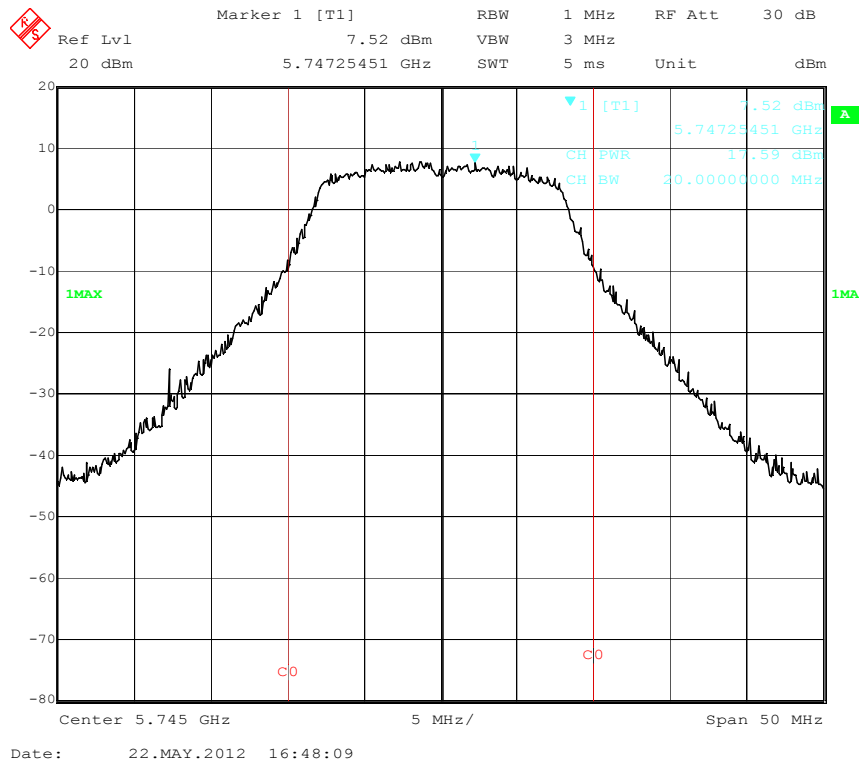
Output Power Low Channel (802.11a)
