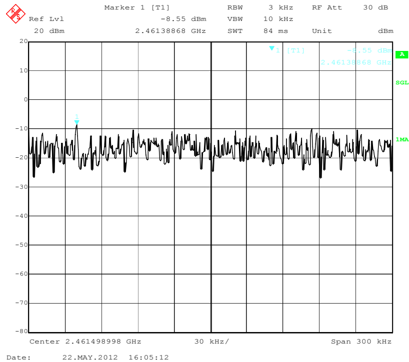
PSD High Channel ( 802.11b)
