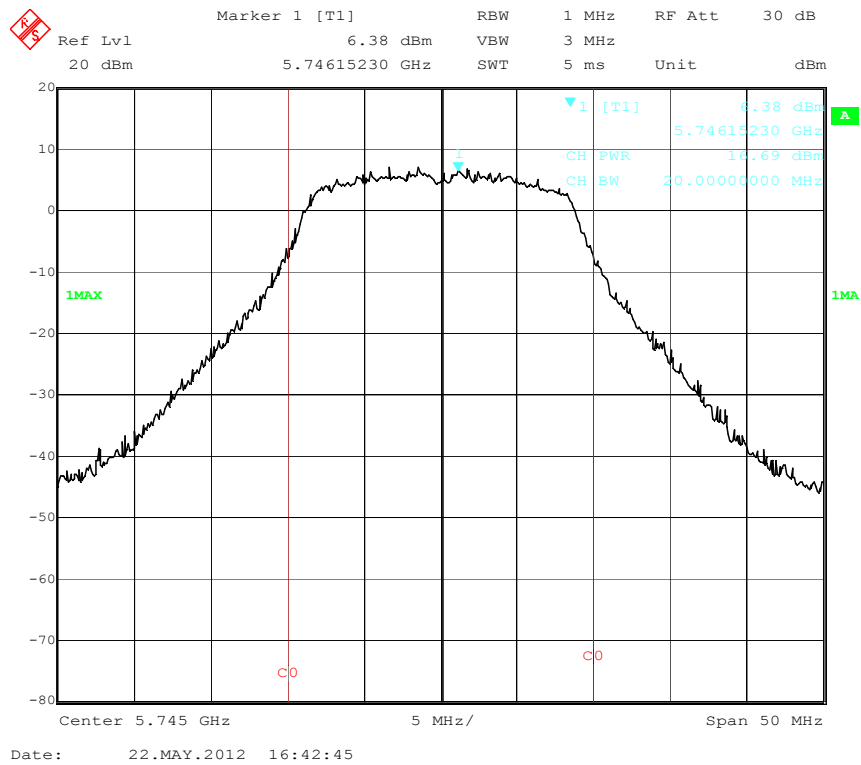
Output Power Low Channel ( 802.11n-20MHz 5.7GHz)
