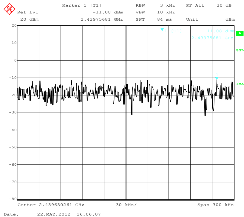
PSD Mid Channel ( 802.11b)
