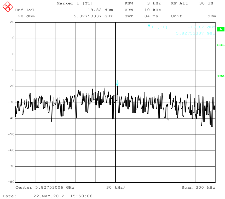
PSD High Channel (802.11n-20MHz 5.7GHz)
