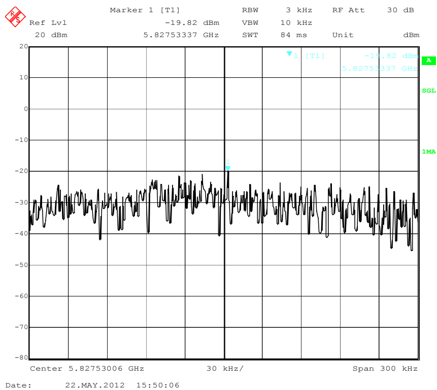
PSD High Channel (802.11a 5.7GHz)
