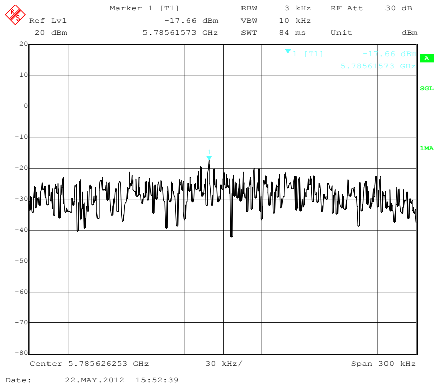
PSD Mid Channel (802.11a 5.7GHz)
