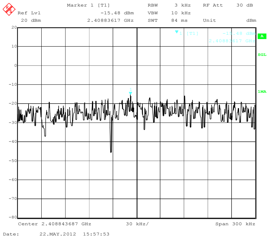
PSD Low Channel ( 802.11g)
