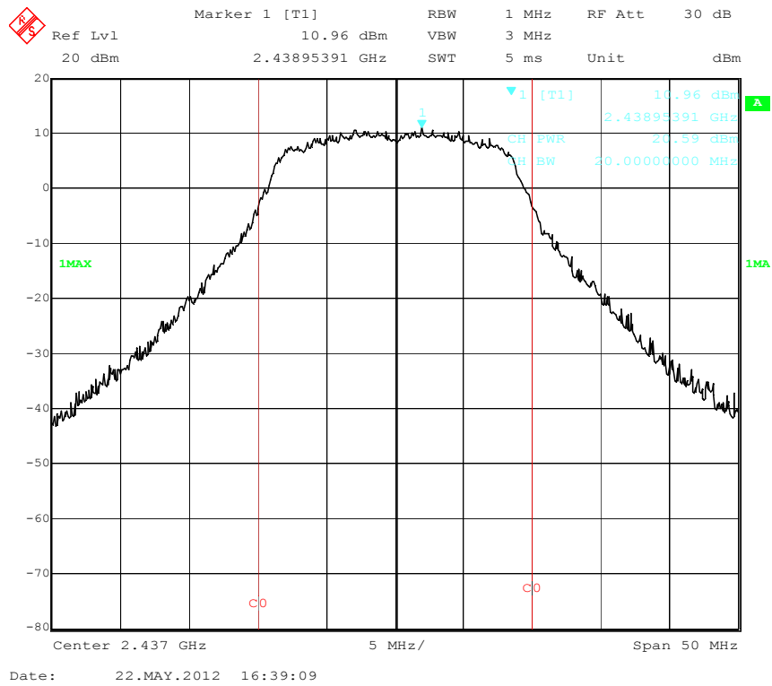
Output Power Middle Channel (802.11n-20MHz)
