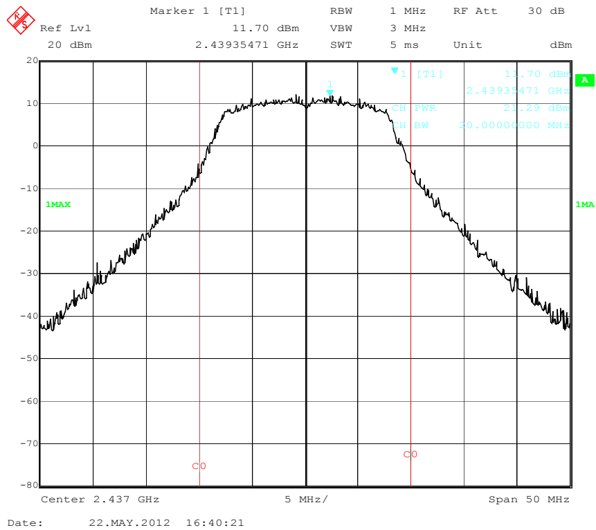
Output Power Middle Channel (802.11g)
