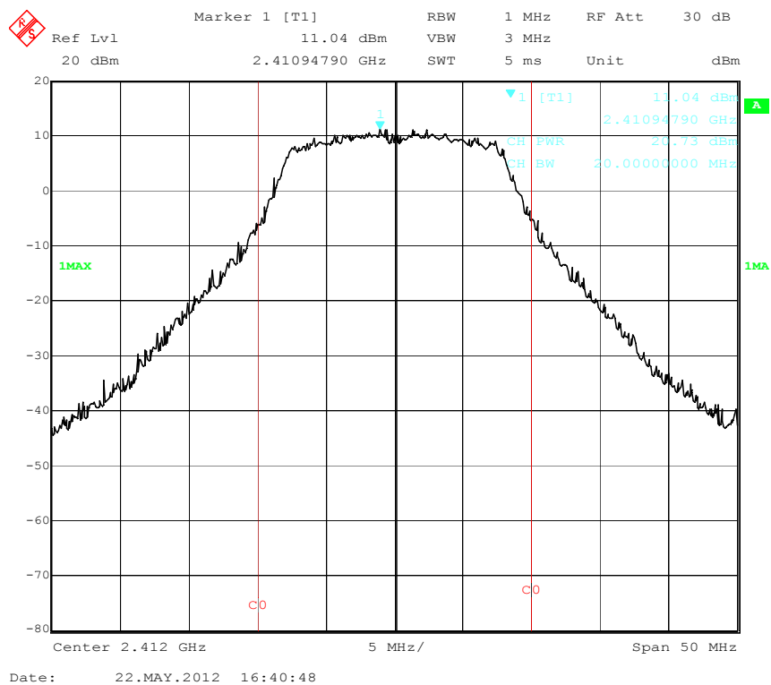
Output Power Low Channel (802.11g)
