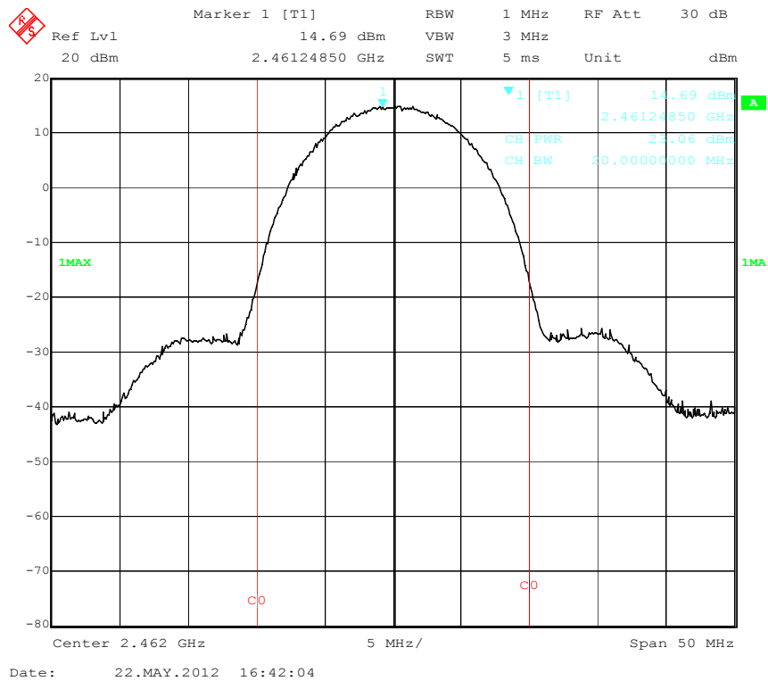
Output Power High Channel (802.11b)
