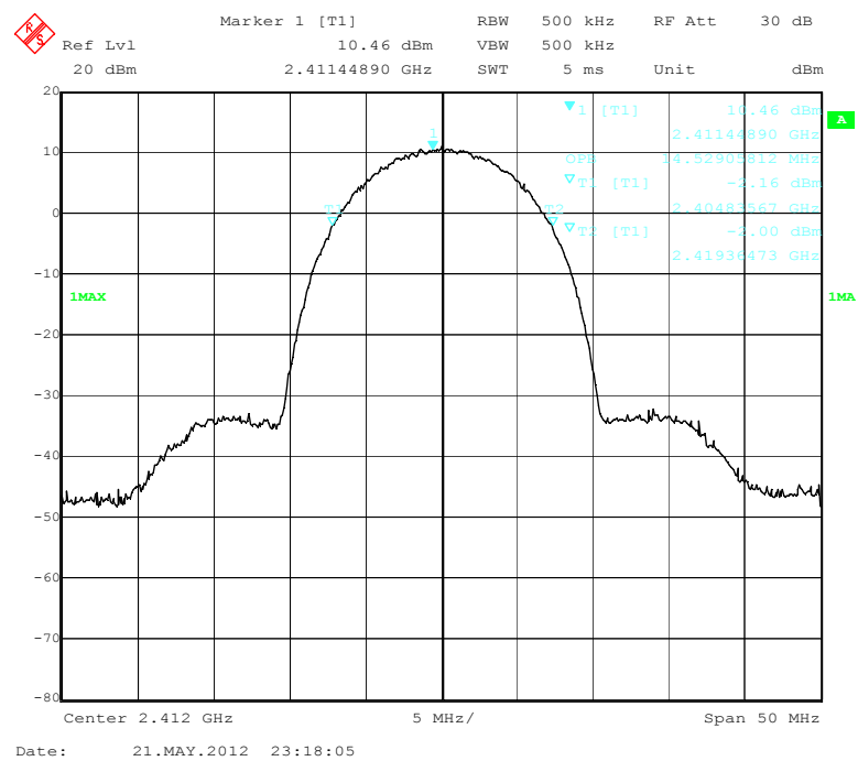
99% dB Bandwidth - 802.11b, Low Channel
