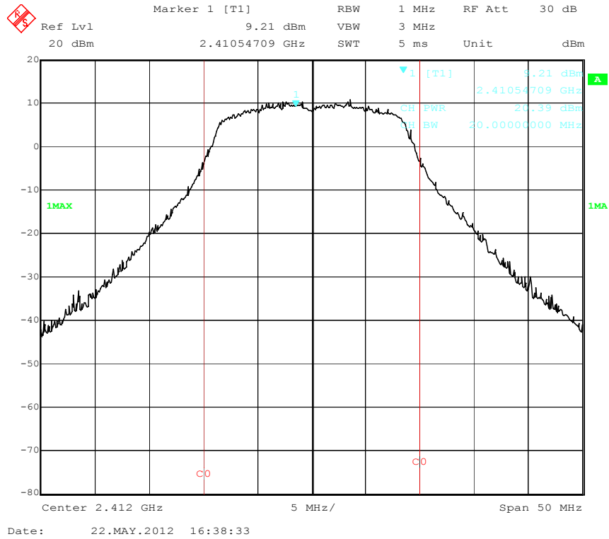
Output Power Low Channel (802.11n-20MHz)
