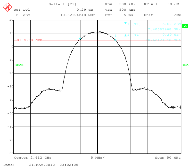
6 dB Bandwidth – 802.11b, Low Channel
