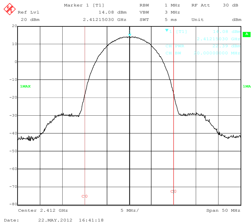
Output Power Low Channel (802.11b)
