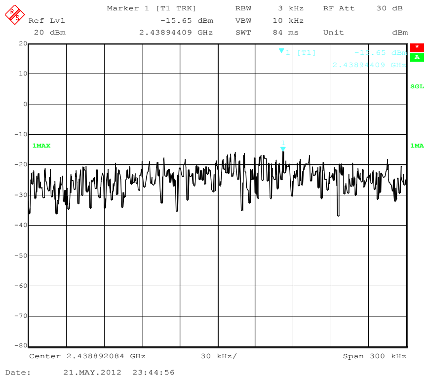
PSD Mid Channel (802.11n-20MHz-2.4G)
