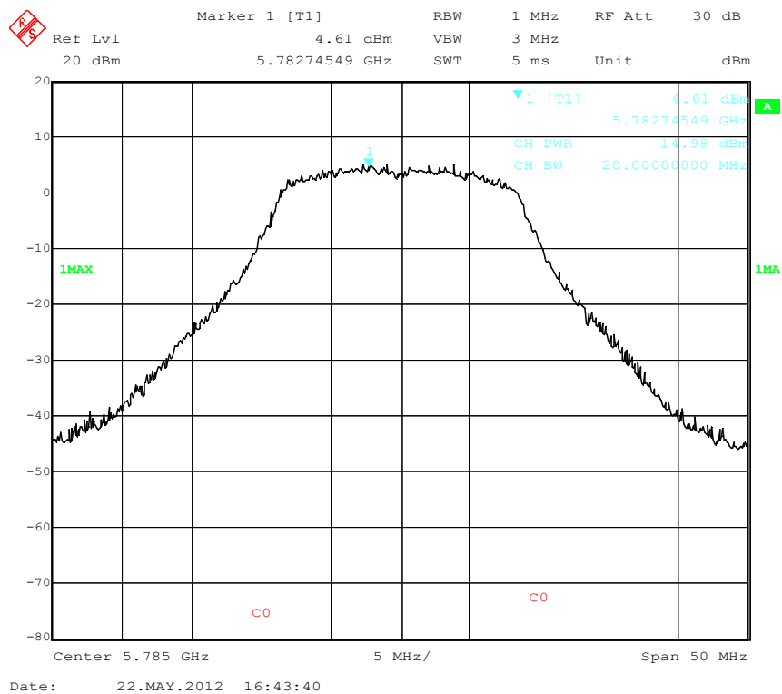
Output Power Mid Channel (802.11n-20MHz 5.7GHz)
