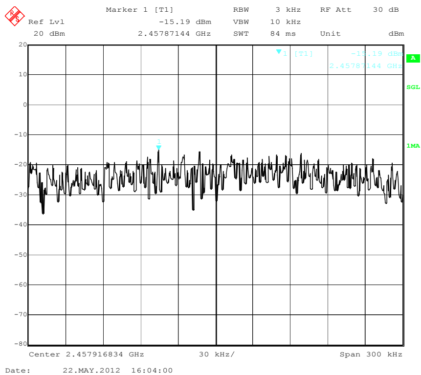
PSD High Channel ( 802.11g)
