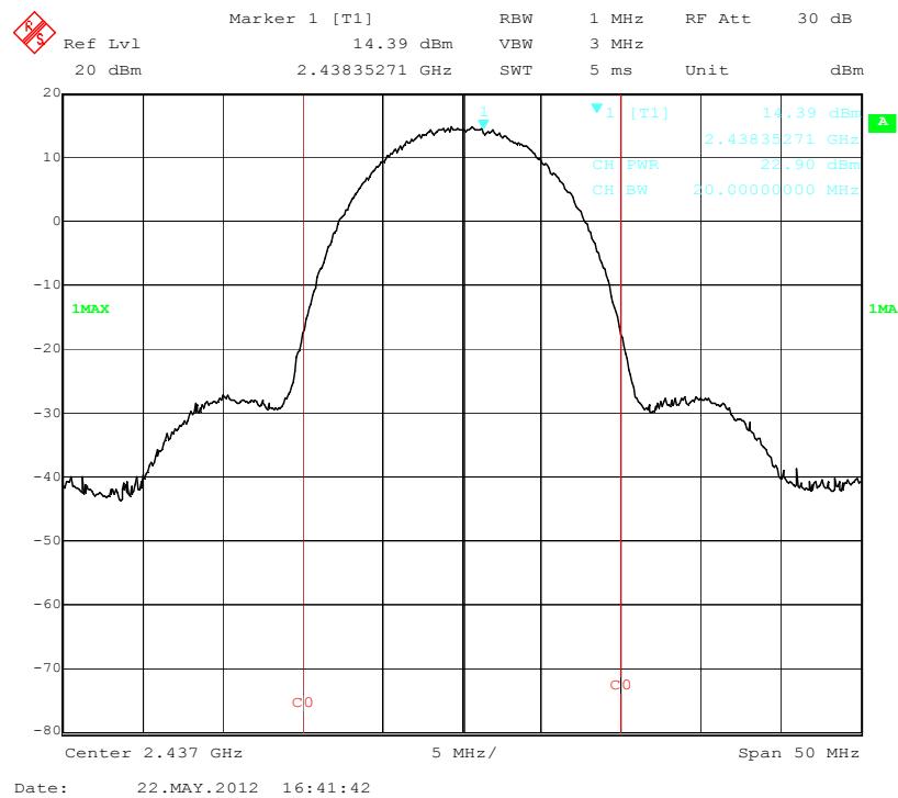
Output Power Middle Channel (802.11b)
