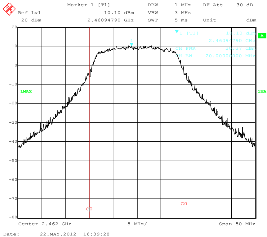
Output Power High Channel (802.11n-20MHz)
