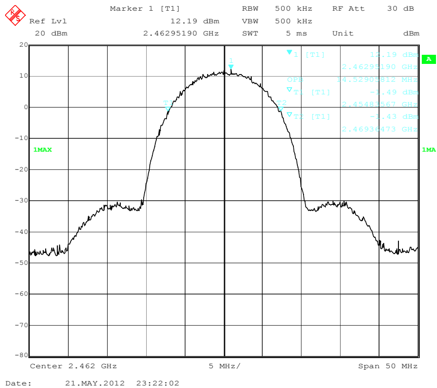
99% dB Bandwidth - 802.11b, High Channel
