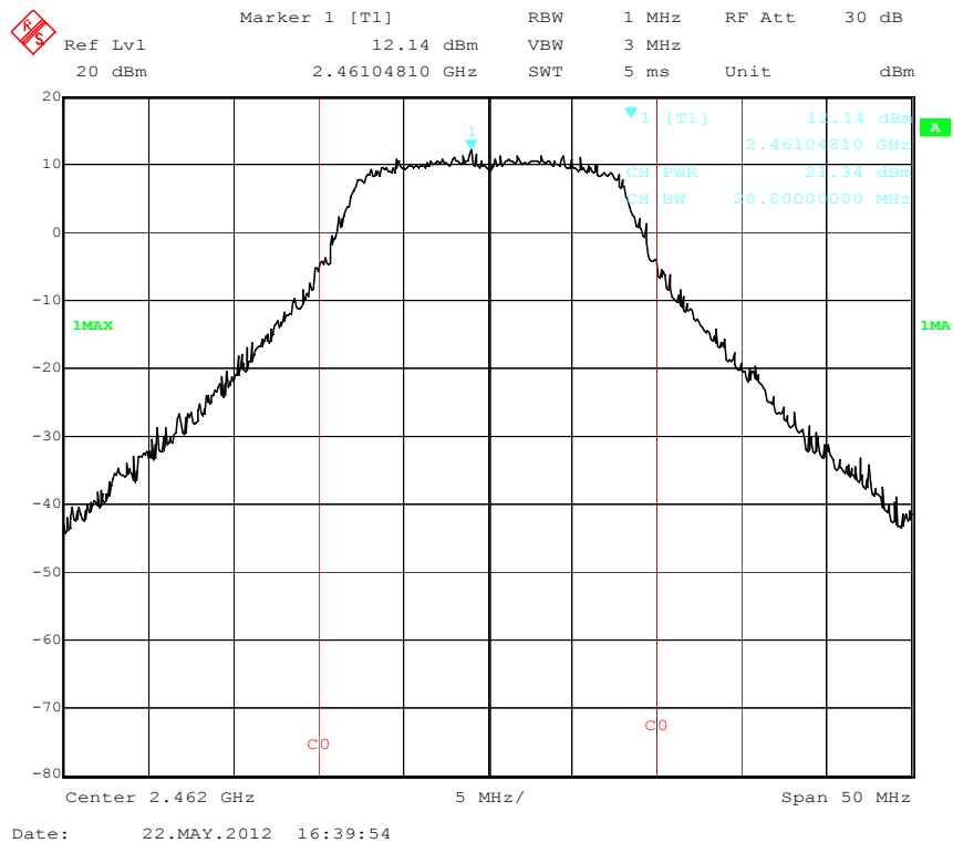
Output Power High Channel (802.11g)
