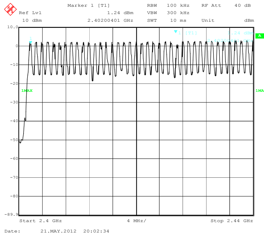
Number of Hopping Channel 39-Channel (Graph 1)
