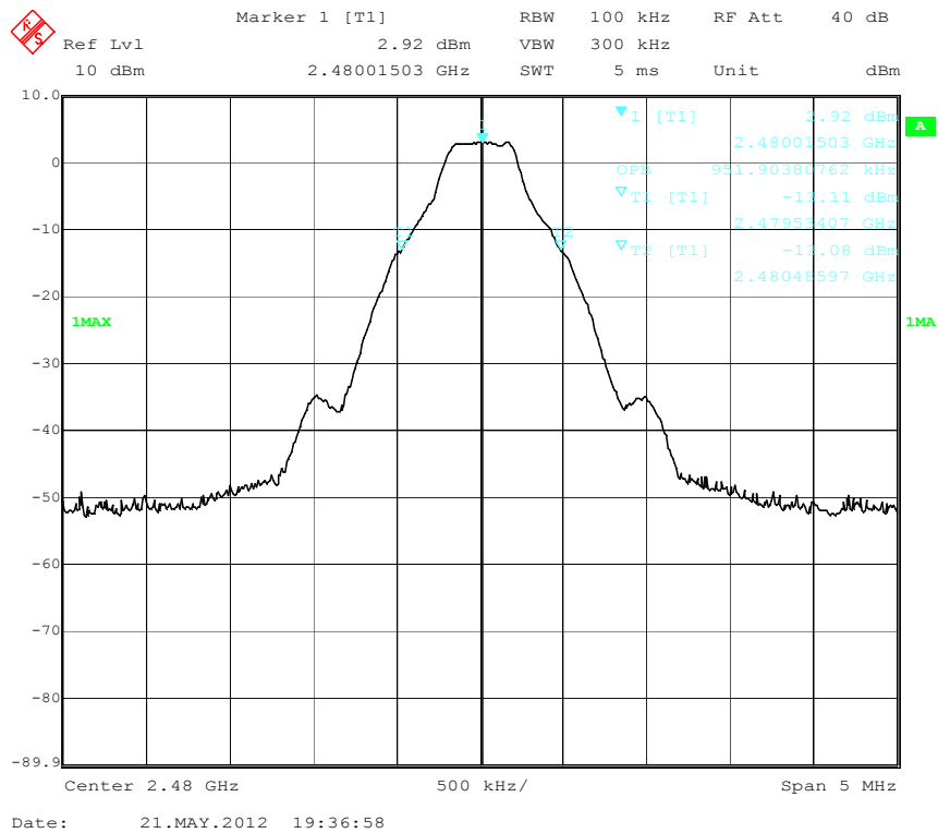
99% dB Bandwidth - High Channel
