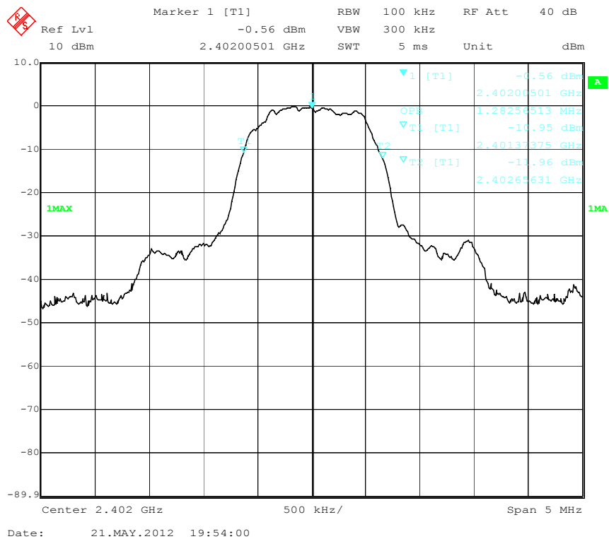
99% dB Bandwidth - Low Channel
