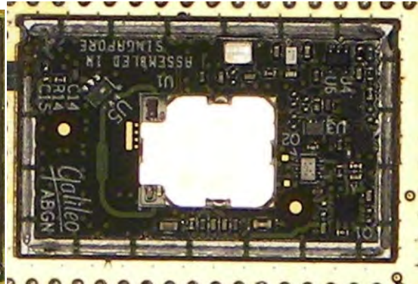
Radio module without shield
