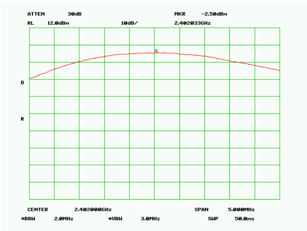
Output Power Low Channel (Bluetooth)
