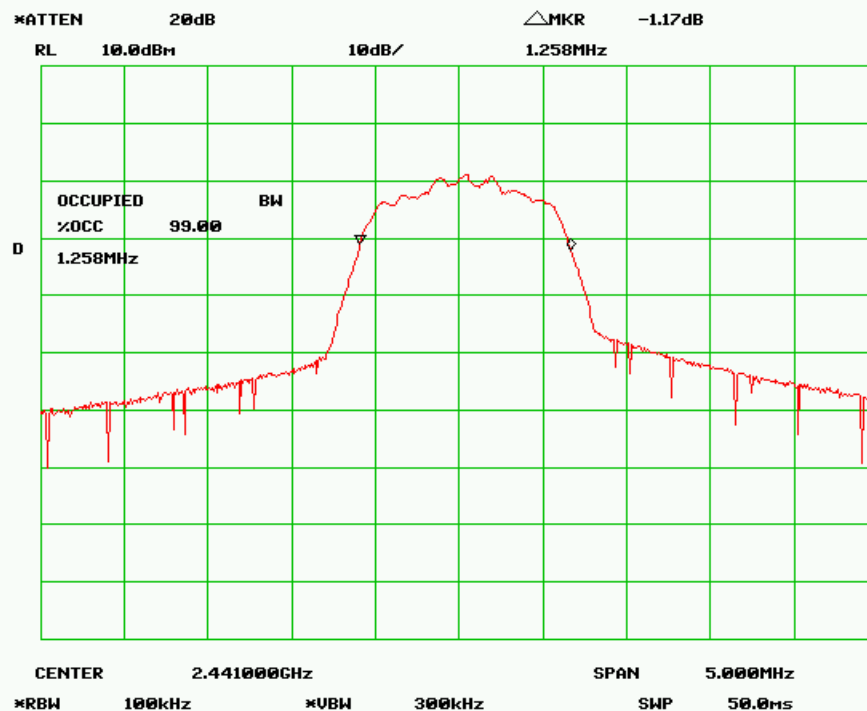
99% dB Bandwidth - Mid Channel
