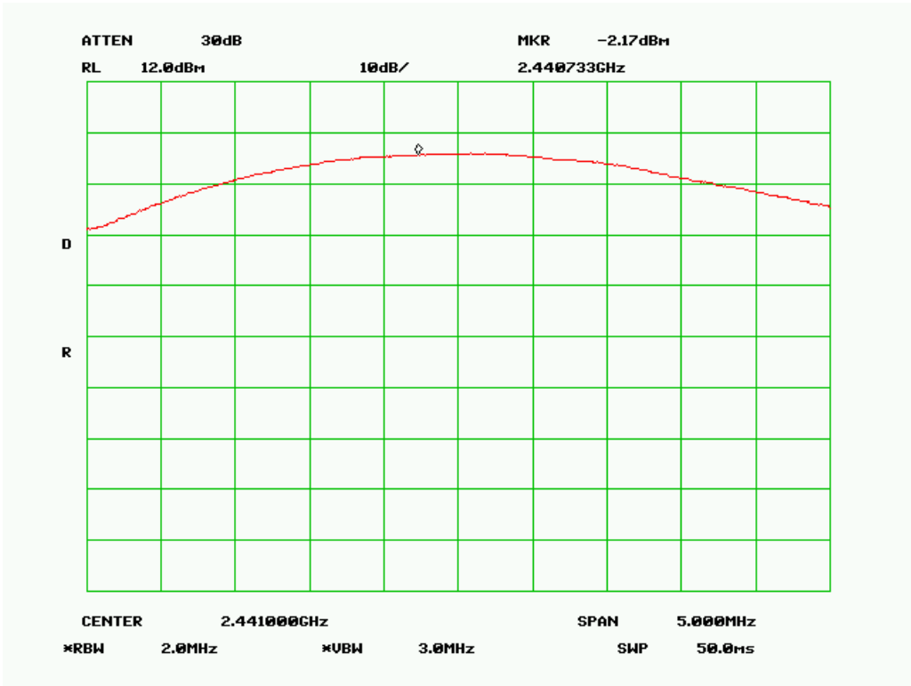
Output Power Middle Channel (Bluetooth)
