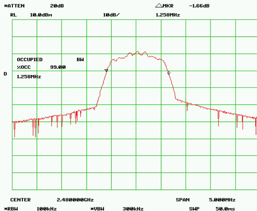
99% dB Bandwidth - High Channel
