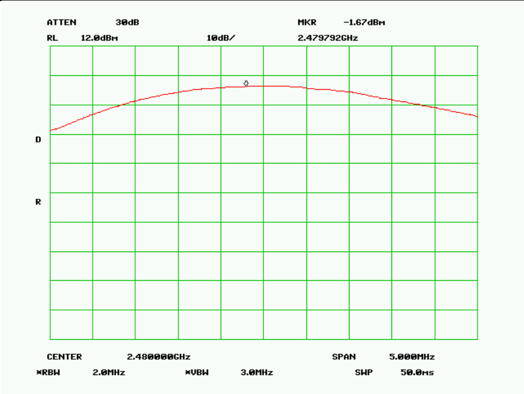
Output Power High Channel (Bluetooth)
