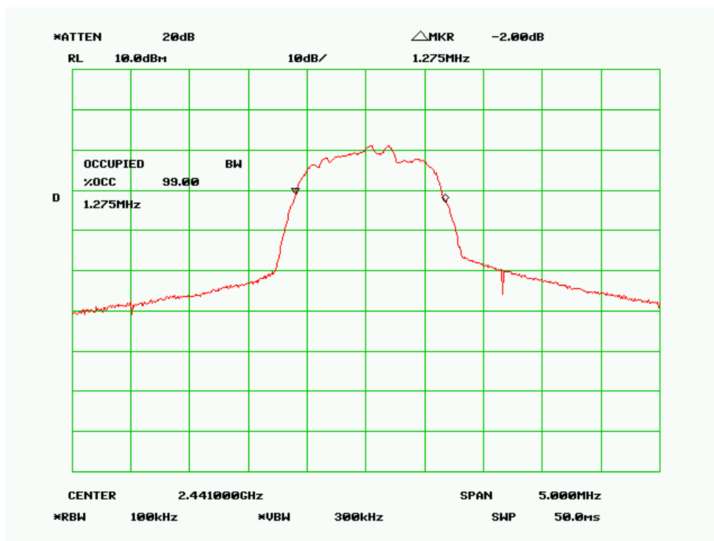
99% dB Bandwidth - Mid Channel
