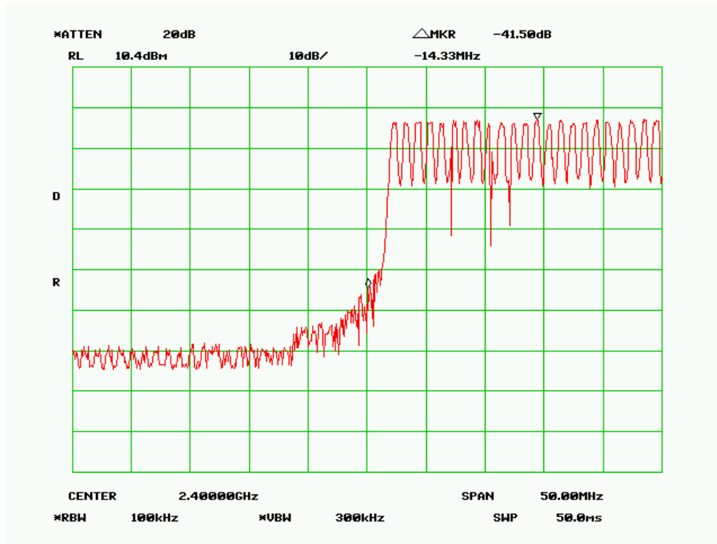
Low Channel
