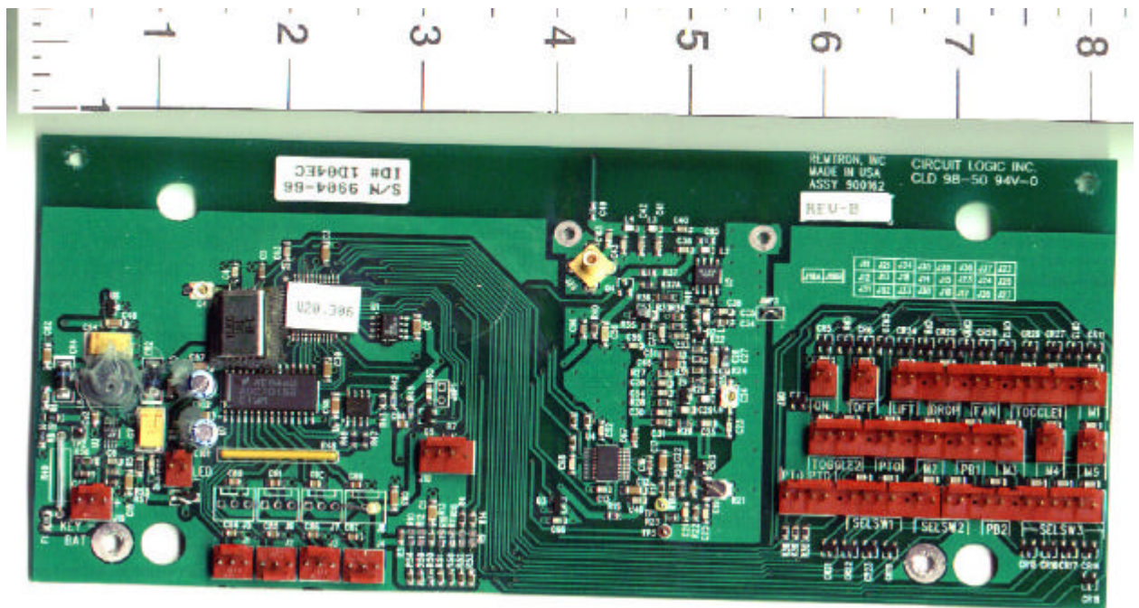
Front and Back of Belly Box Transmitter 21T34 PCB
