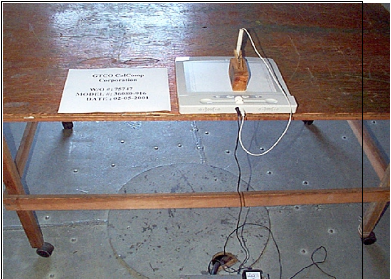
Radiated Emissions - Back View, Horizontal Orthogonal
