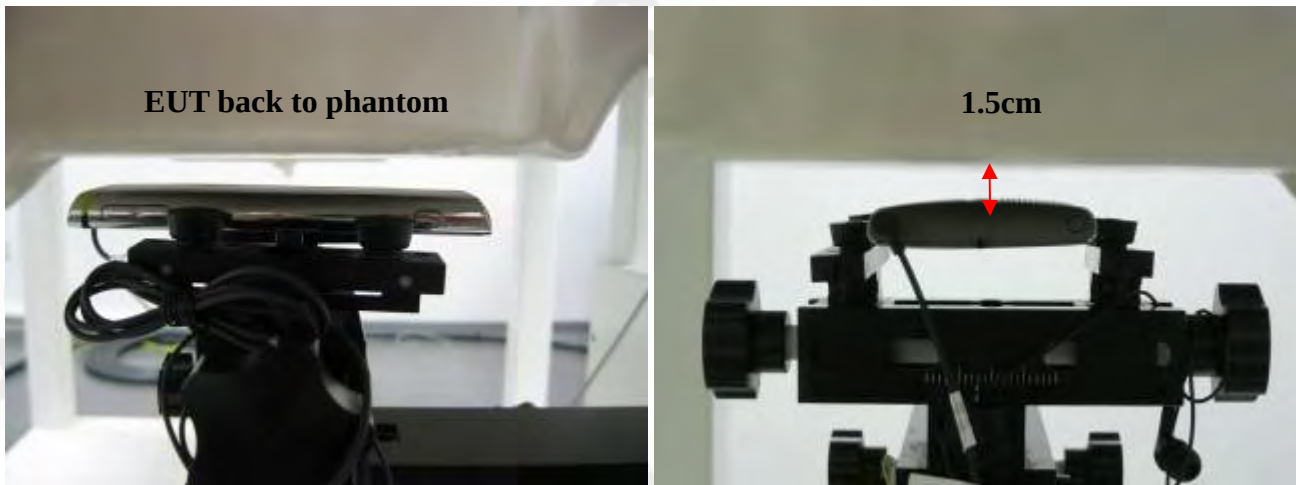
Fig.9 Body worn- EUT back to flat phantom and distance between flat phantom and mobile phone is 1.5 cm (repeated with headset)
