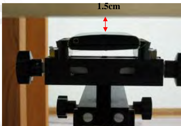
Fig.12 Body worn- EUT back to flat phantom and distance between flat phantom and mobile phone is 1.5 cm
