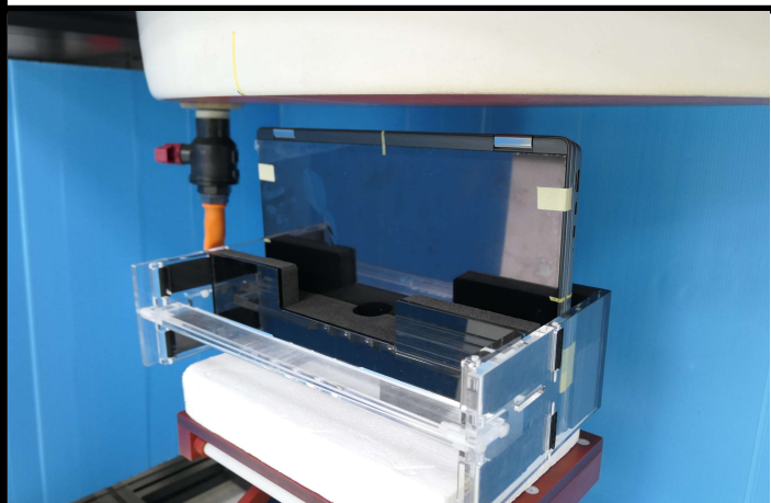
Bottom Side of Tablet Mode Test at 19 mm
