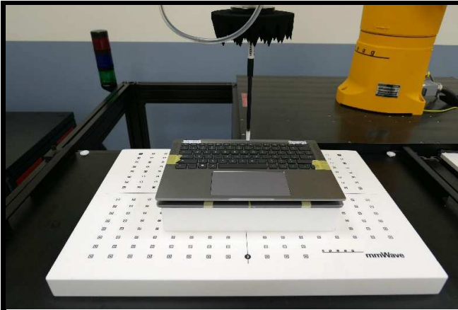
Rear Face of Tablet Mode Test at 0 mm
