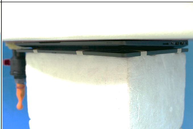
Rear Face of Tablet Mode Tested at 0 mm CF Material of Cover
