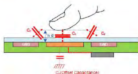
Figure 3. Case of GND pattern(@1/3d distance)
