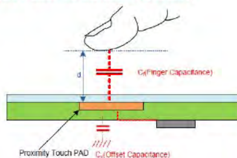
Figure 1. Case of No-GND pattern(@d distance)
