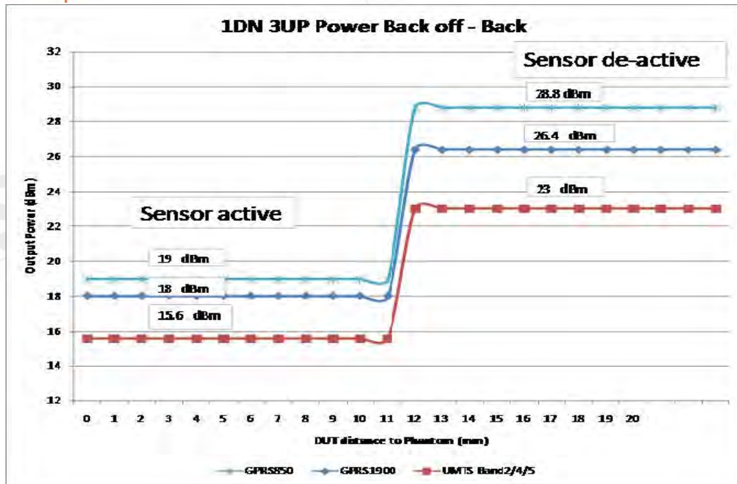
Distance vs. output power plot(1DN 3UP)
