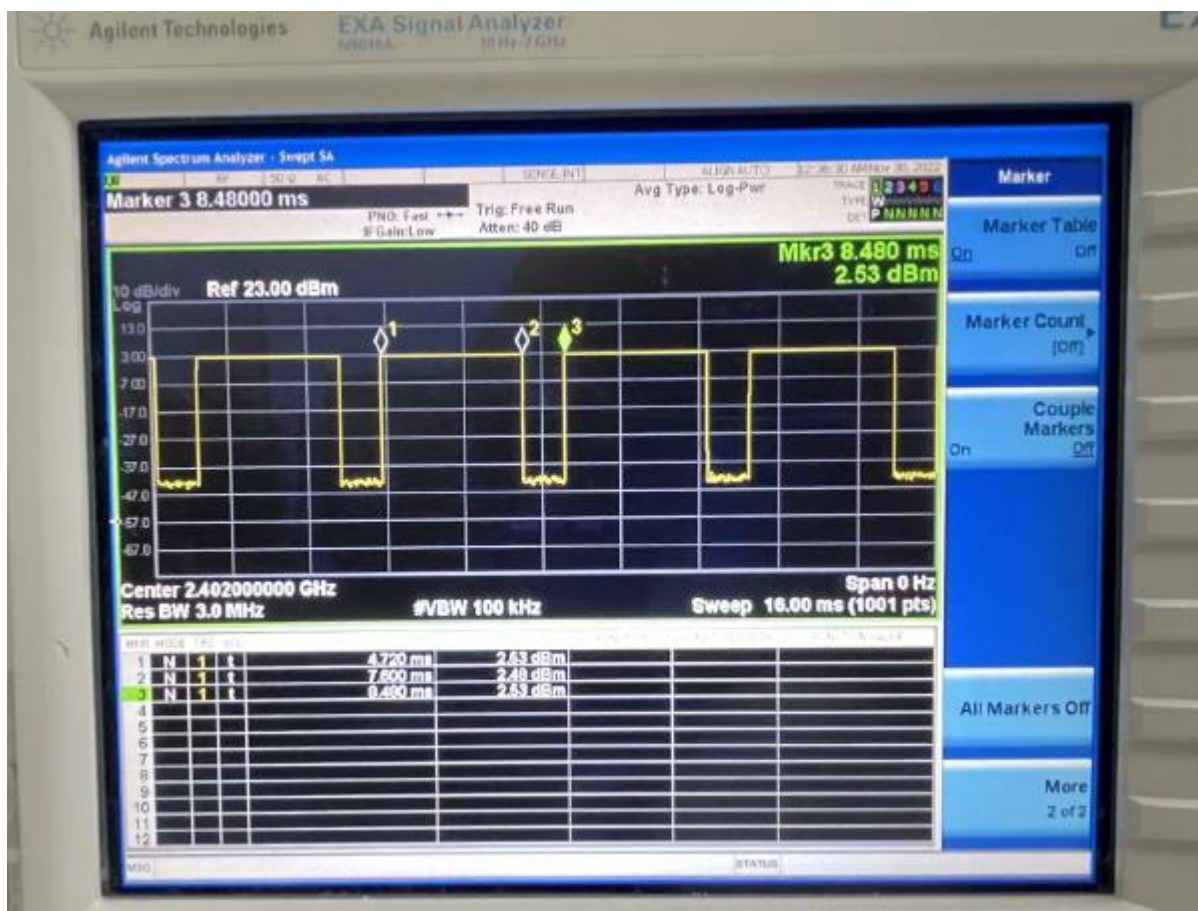
Time-domain plot for Bluetooth transmission signal
