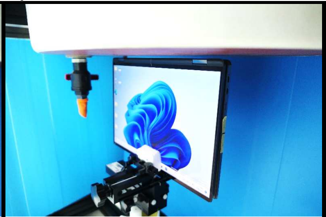
Bottom Side of Tablet Mode Tested at 5 mm
