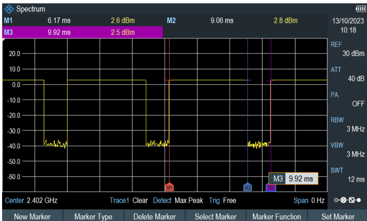
Time-domain plot for Bluetooth transmission signal
