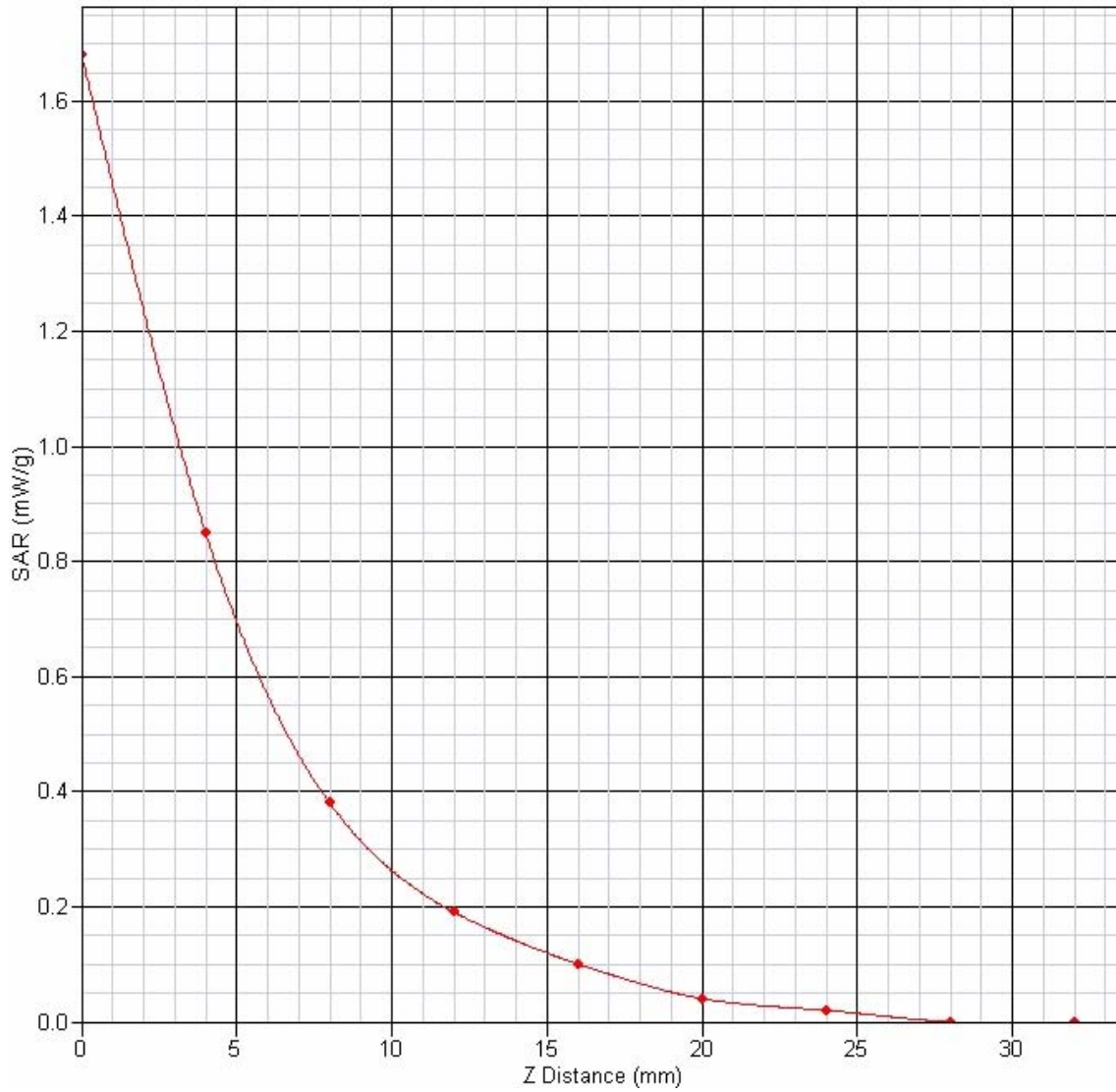
SAR-Z Axis at Hotspot x:0.0 y:0.0
