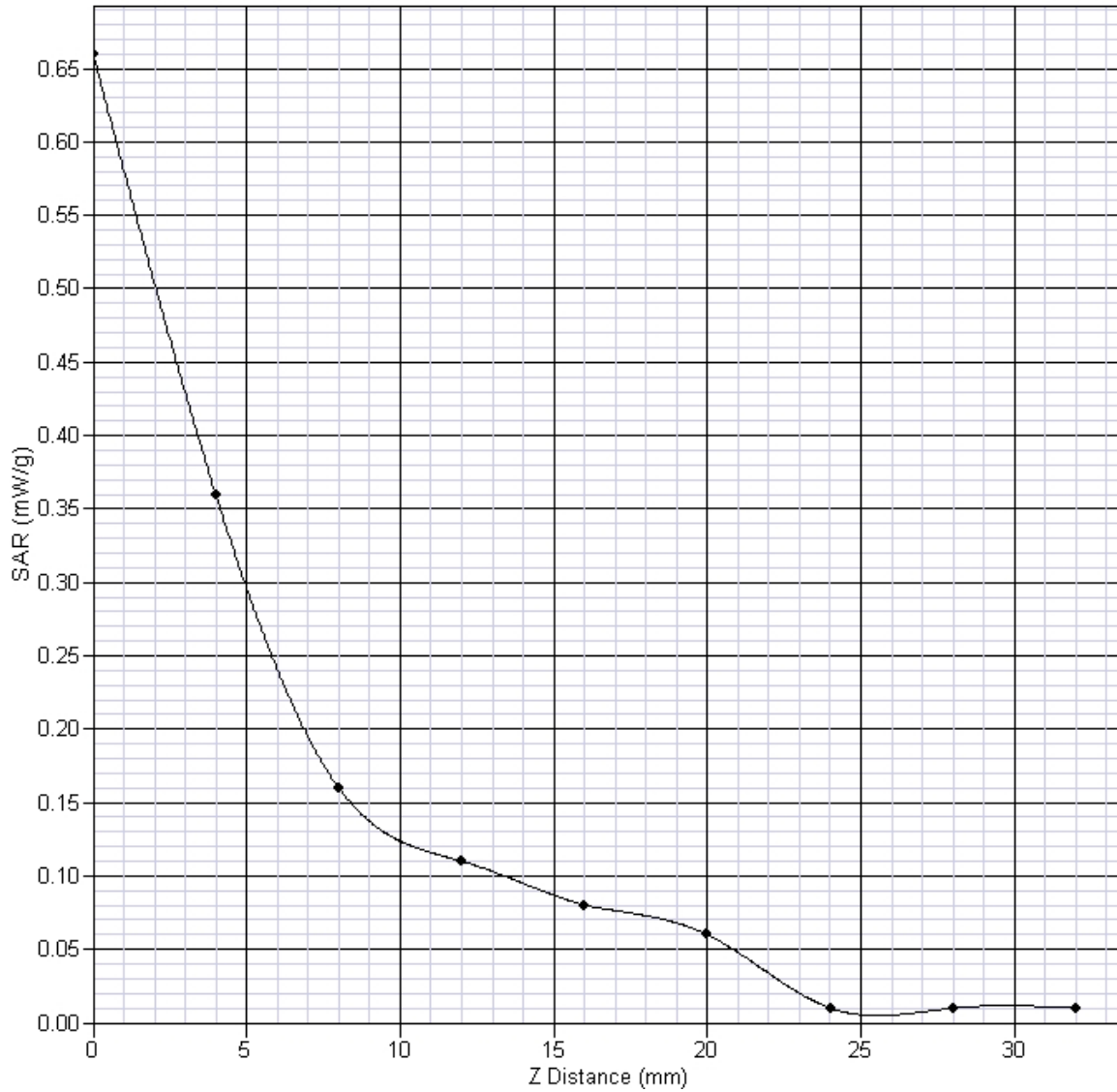
SAR-Z Axis at Hotspot x:38.2 y:26.1
