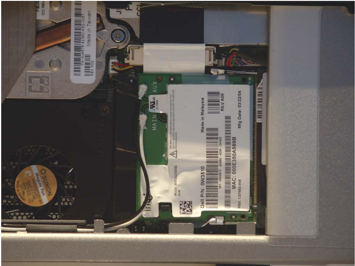
View of the WLAN Transmitter Location Inside the Laptop (Close-Up)
