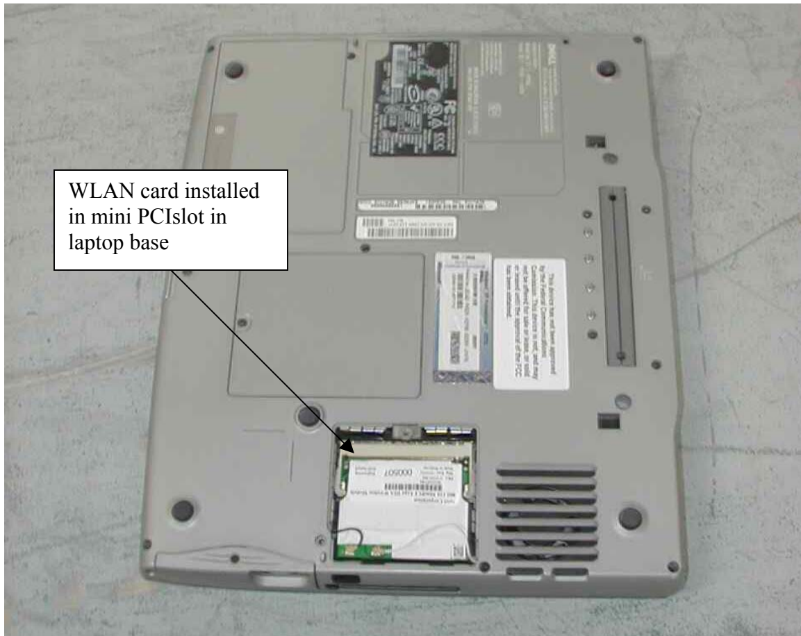
Picture Showing Placement Of 802.11b Card In The Laptop
