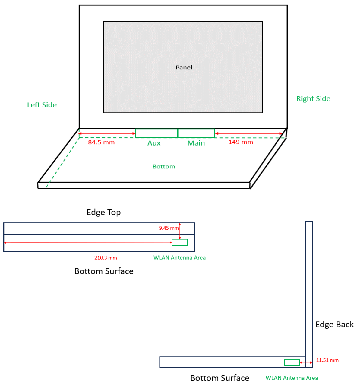
Photograph 15. Antenna position of EUT
