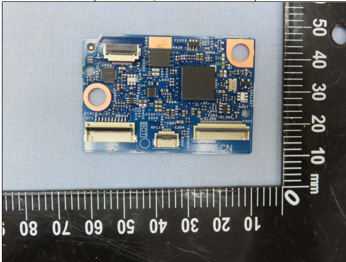
RFID 13.56MHz Wireless Module (Brand: DELL, Model: DWRFID2403)
