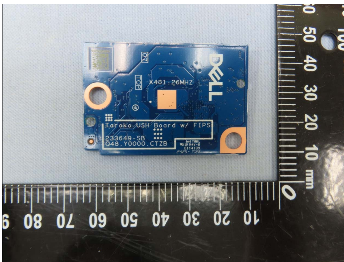
Portable Computer (Brand: DELL, Model: P194G)
