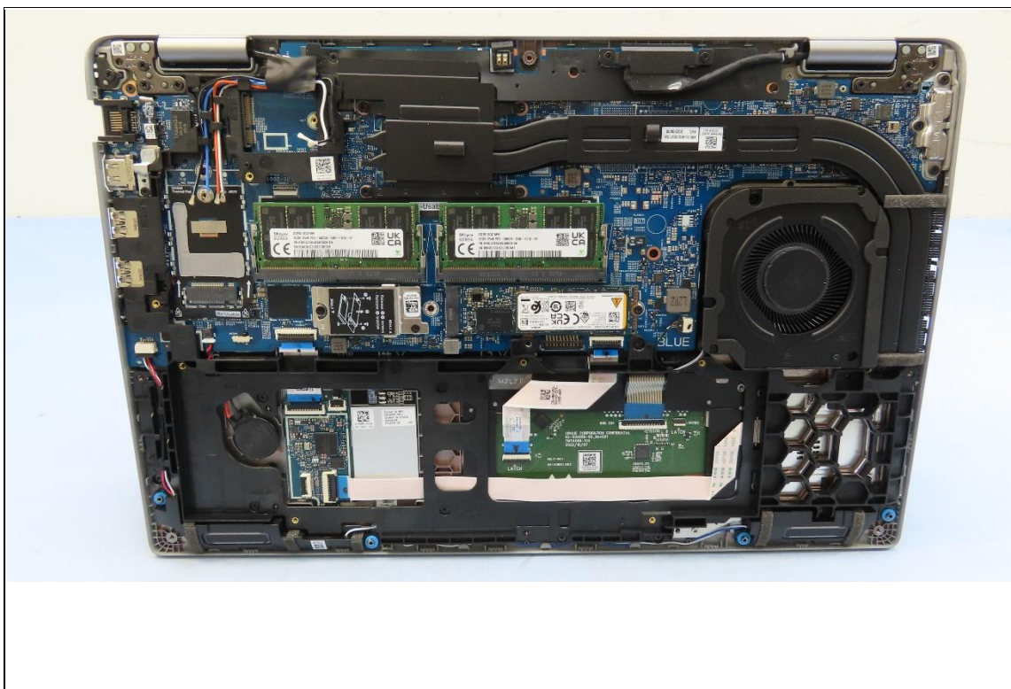
End-product, Portable Computer (Brand: DELL, Model: P127F)
