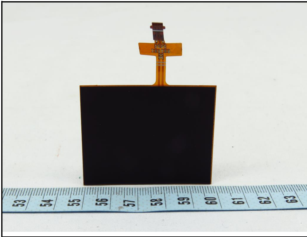
Speedwire Antenna
