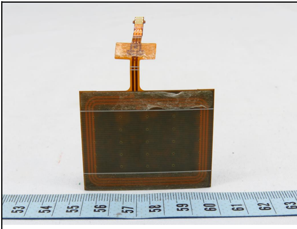
Speedwire Antenna
