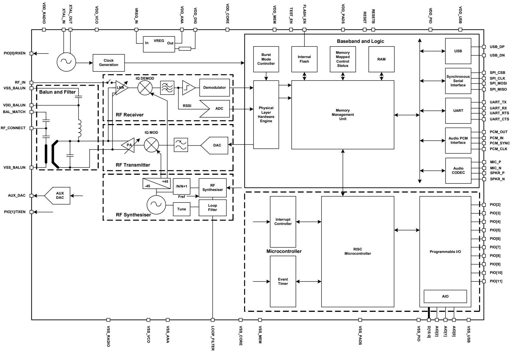
Figure 5.1: BlueCore2-Flash Plug-n-Go Device Diagram for 10 x 10mm LFBGA Package
