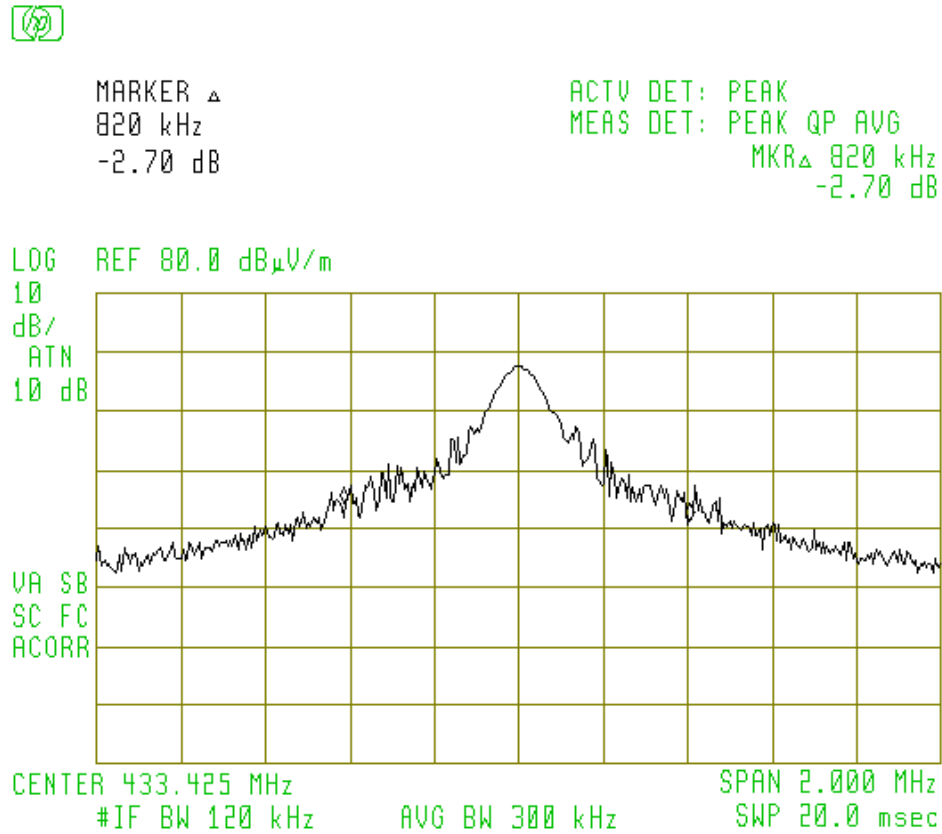
Figure 6.1-2 99% Bandwidth
