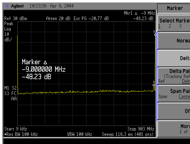
Figure 20. Spurious emission between 9 kHz and 902 MHz is -48.23 dBc.
