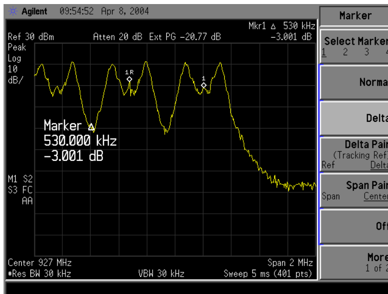
Figure 3. Channel separation at high band is 530 kHz
