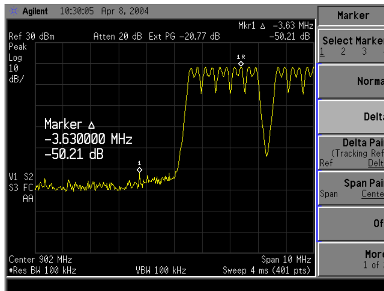
Figure 18. Spurious emission at lower band edge is -50.21 dBc.
