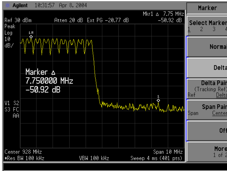
Figure 19. Spurious emission at upper band edge is -50.92 dBc.
