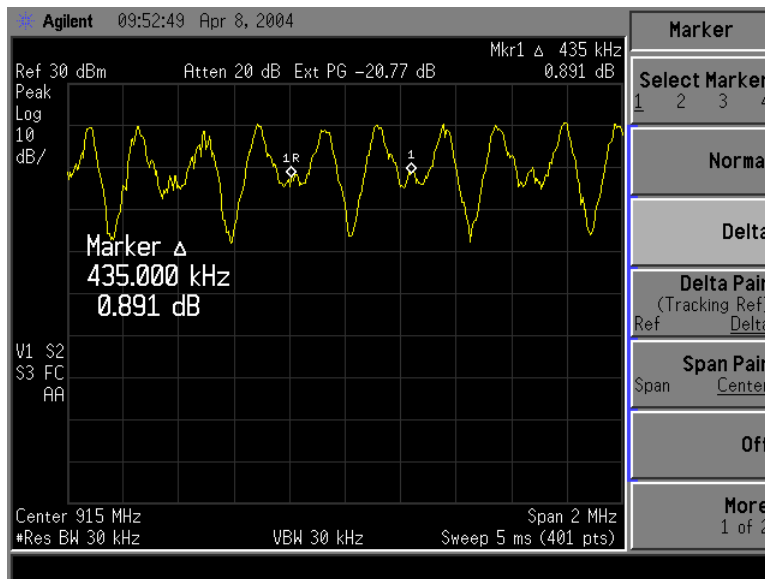
Figure 2. Channel separation at mid band is 435 kHz
