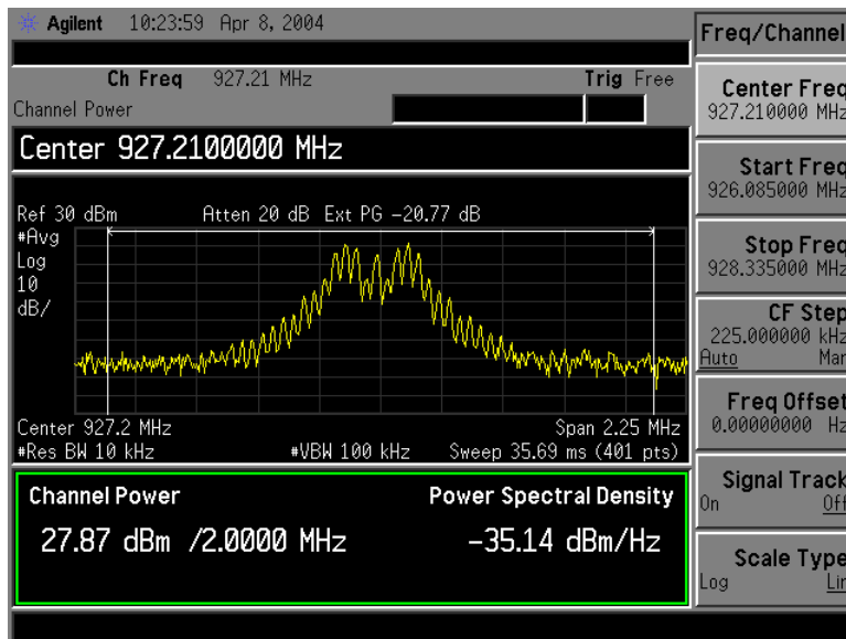
Figure 17. Highest channel power is +27.87 dBm on highest channel at 3.0 volt supply input.
