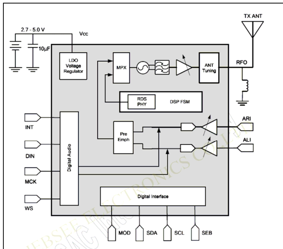
FM Transmitter IC
