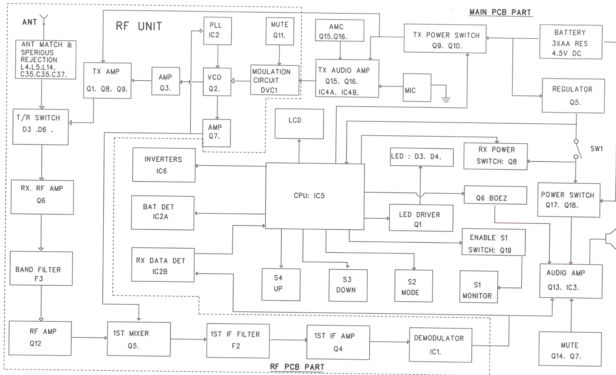
BLOCK DIAGRAM (FRS-0128)
