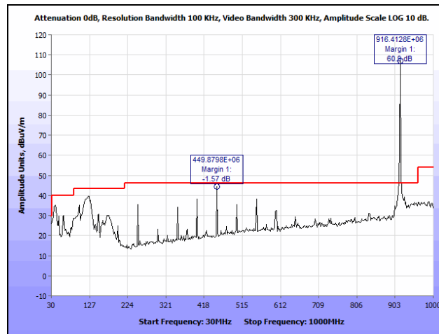
Plot 4. Radiated Spurious Emissions, Mid Channel, 30 MHz – 1 GHz
