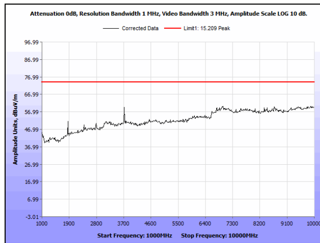
Plot 9. Radiated Spurious Emissions, High Channel, Peak, 1 GHz – 10 GHz
