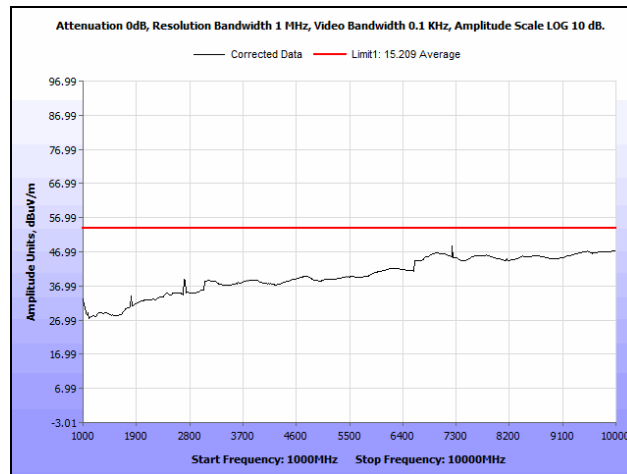
Plot 2. Radiated Spurious Emissions, Low Channel, Average, 1 GHz – 10 GHz
