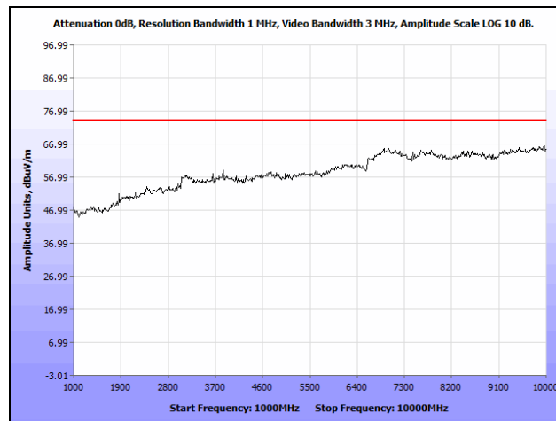
Plot 6. Radiated Spurious Emissions, Mid Channel, Peak, 1 GHz – 10 GHz
