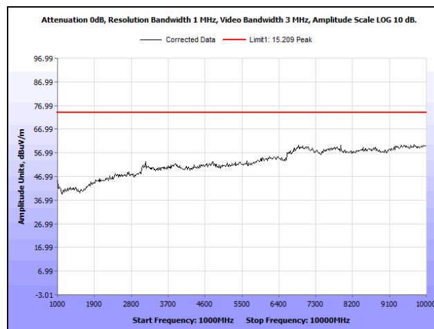
Plot 3. Radiated Spurious Emissions, Low Channel, Peak, 1 GHz – 10 GHz
