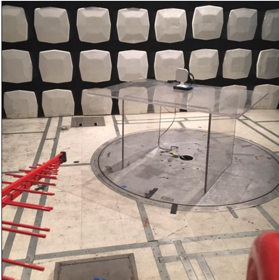
Photograph 2. Radiated Spurious Emissions, Test Setup
